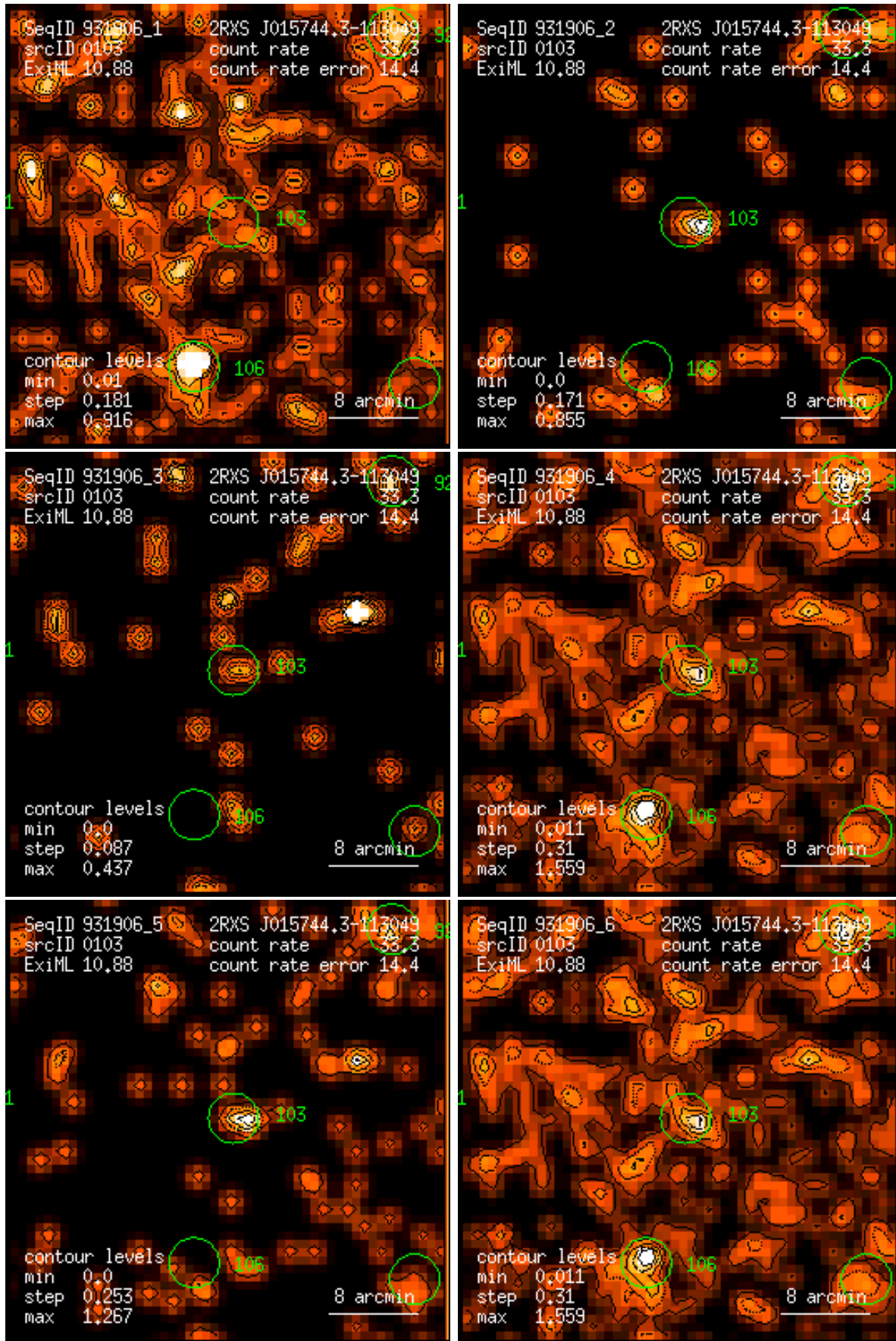
Figure 103: RASS 931906: detection 0103: band rate images, Gaussian filter: (1) PSPC channels 11 – 41, (2) 52 – 90, (3) 91 – 201, (4) 11 – 235, (5) 52 – 201, (6) 11 – 201. Broad band rates in counts/ks. Band rate contour levels in counts/ks/arcmin 2 .
