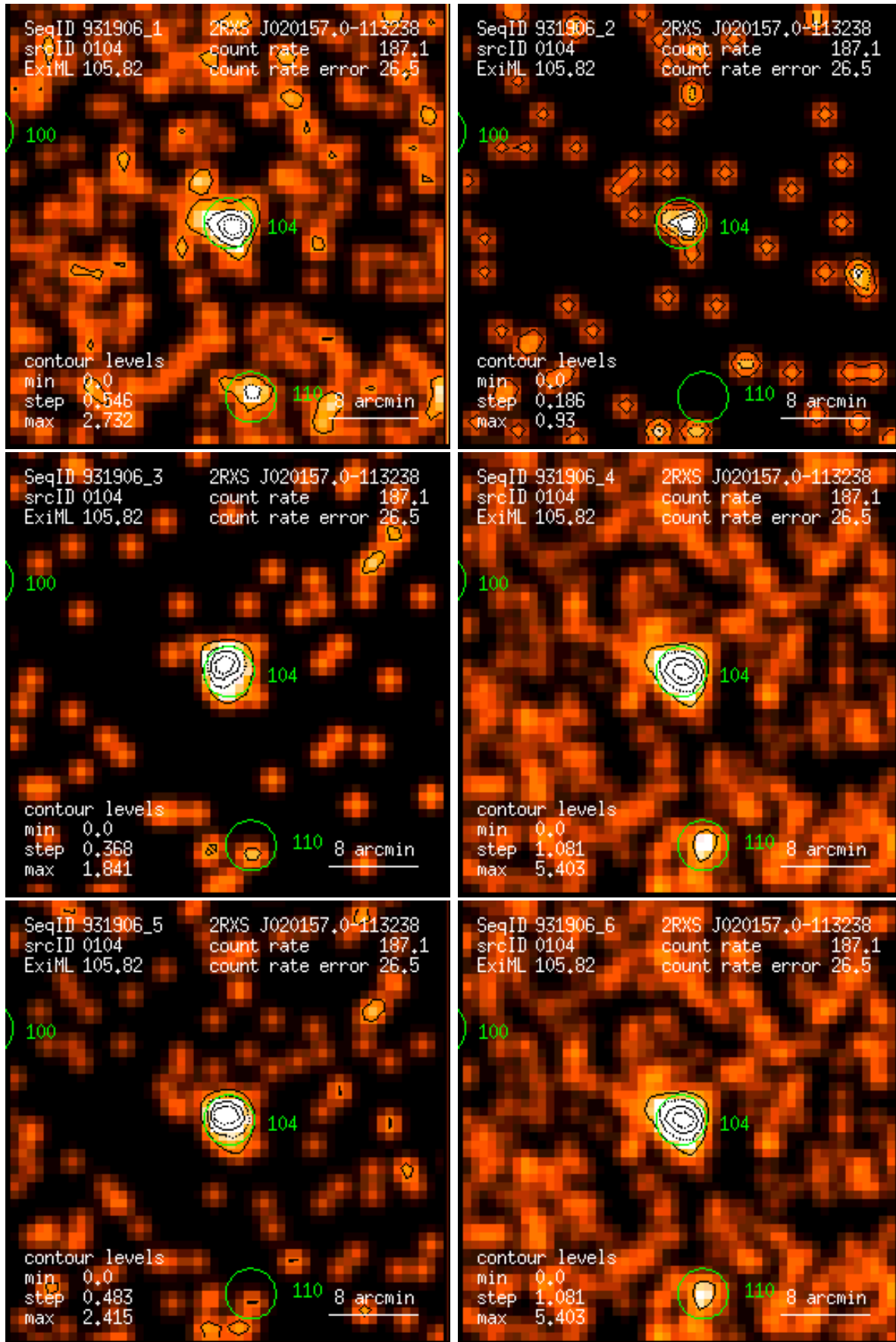
Figure 104: RASS 931906: detection 0104: band rate images, Gaussian filter: (1) PSPC channels 11 – 41, (2) 52 – 90, (3) 91 – 201, (4) 11 – 235, (5) 52 – 201, (6) 11 – 201. Broad band rates in counts/ks. Band rate contour levels in counts/ks/arcmin 2 .
