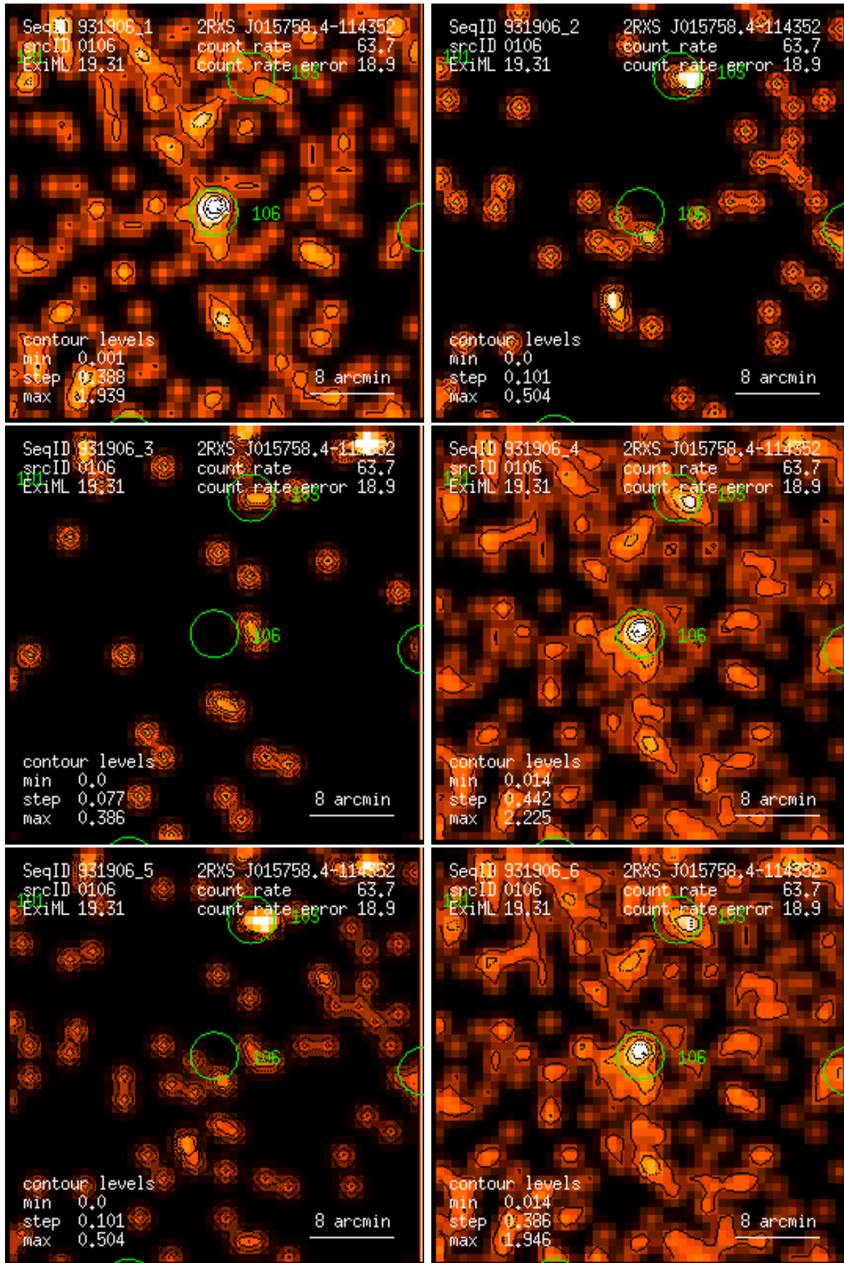
Figure 106: RASS 931906: detection 0106: band rate images, Gaussian filter: (1) PSPC channels 11 – 41, (2) 52 – 90, (3) 91 – 201, (4) 11 – 235, (5) 52 – 201, (6) 11 – 201. Broad band rates in counts/ks. Band rate contour levels in counts/ks/arcmin 2 .
