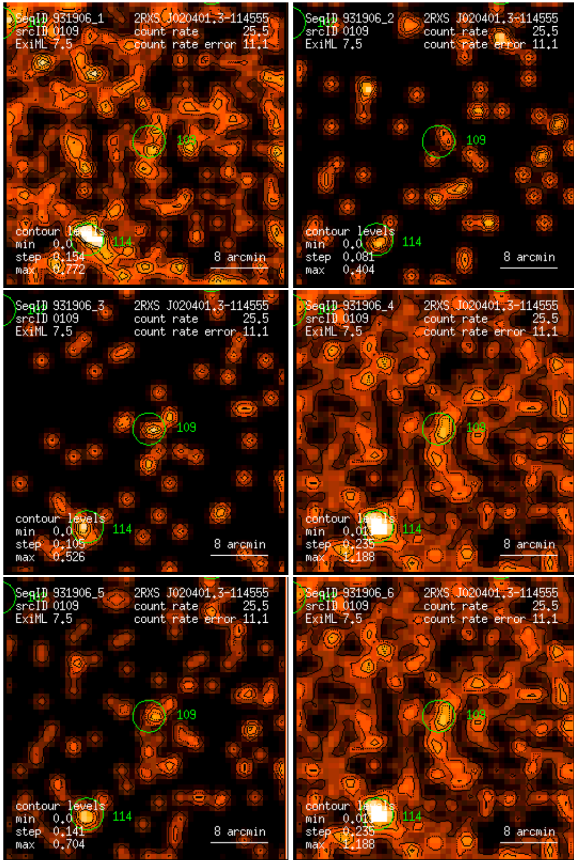
Figure 109: RASS 931906: detection 0109: band rate images, Gaussian filter: (1) PSPC channels 11 – 41, (2) 52 – 90, (3) 91 – 201, (4) 11 – 235, (5) 52 – 201, (6) 11 – 201. Broad band rates in counts/ks. Band rate contour levels in counts/ks/arcmin 2 .
