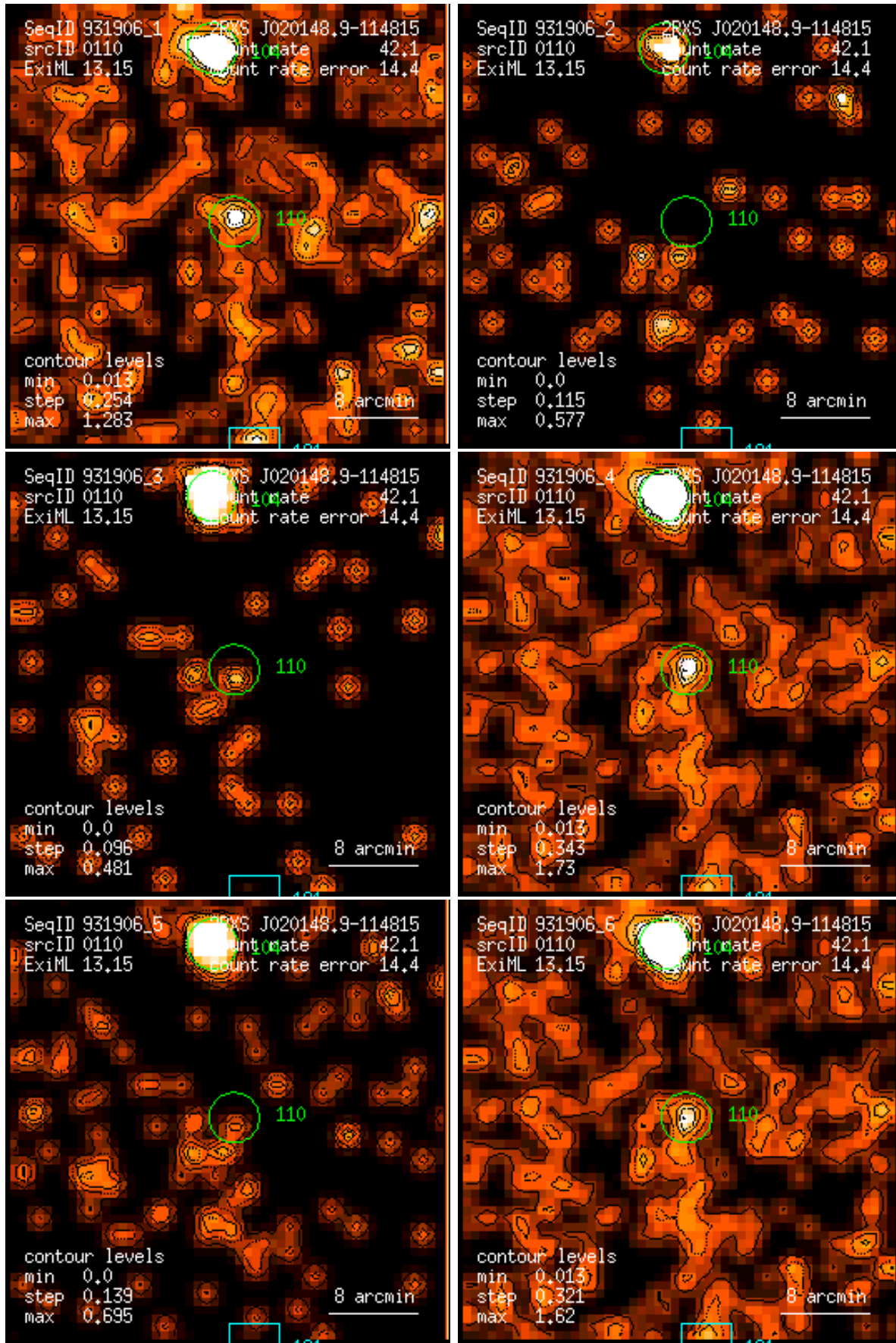
Figure 110: RASS 931906: detection 0110: band rate images, Gaussian filter: (1) PSPC channels 11 – 41, (2) 52 – 90, (3) 91 – 201, (4) 11 – 235, (5) 52 – 201, (6) 11 – 201. Broad band rates in counts/ks. Band rate contour levels in counts/ks/arcmin 2 .
