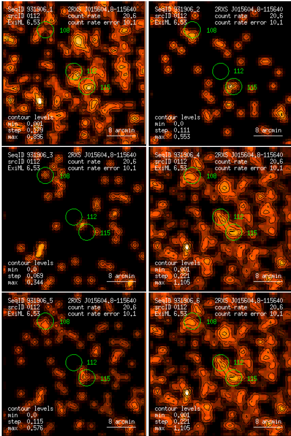
Figure 112: RASS 931906: detection 0112: band rate images, Gaussian filter: (1) PSPC channels 11 – 41, (2) 52 – 90, (3) 91 – 201, (4) 11 – 235, (5) 52 – 201, (6) 11 – 201. Broad band rates in counts/ks. Band rate contour levels in counts/ks/arcmin 2 .
