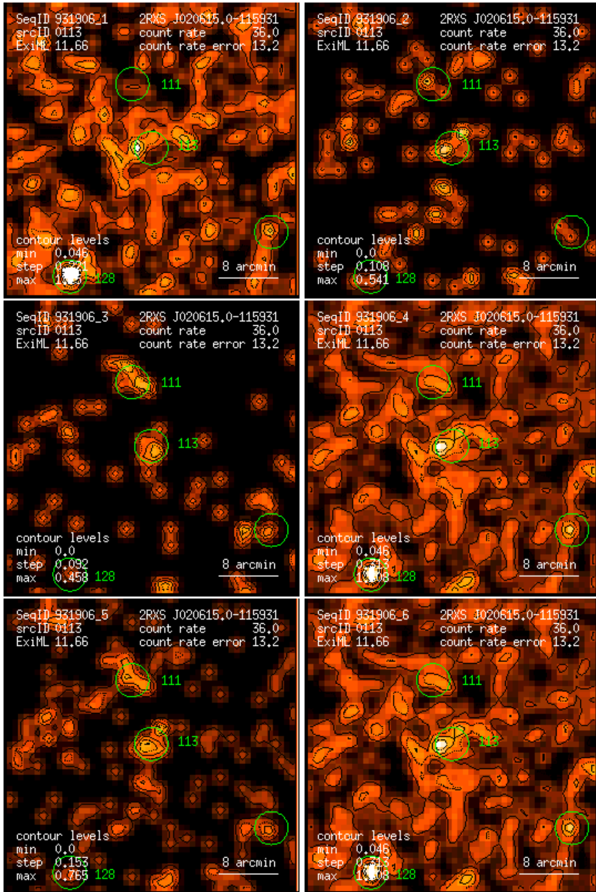
Figure 113: RASS 931906: detection 0113: band rate images, Gaussian filter: (1) PSPC channels 11 – 41, (2) 52 – 90, (3) 91 – 201, (4) 11 – 235, (5) 52 – 201, (6) 11 – 201. Broad band rates in counts/ks. Band rate contour levels in counts/ks/arcmin 2 .
