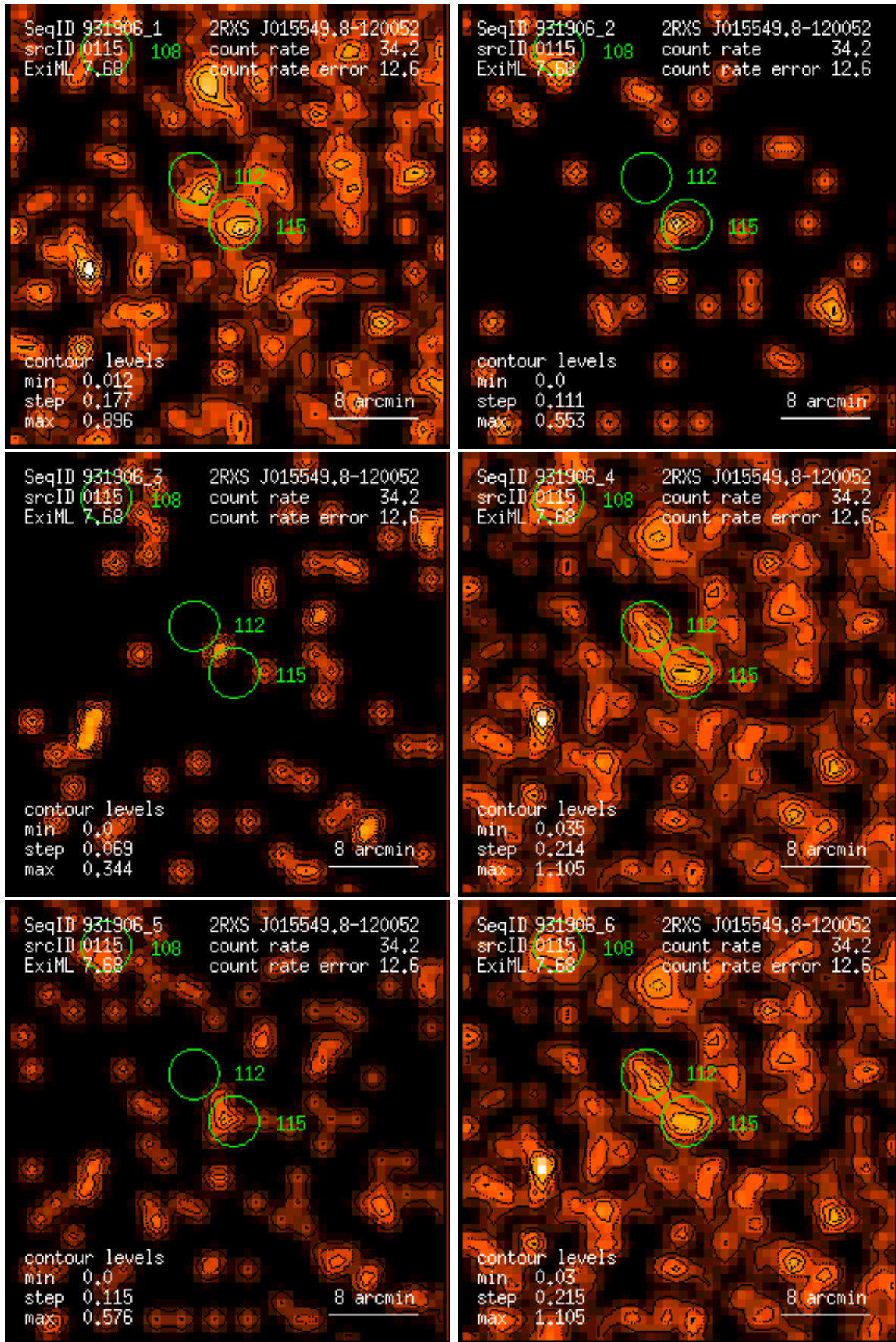
Figure 115: RASS 931906: detection 0115: band rate images, Gaussian filter: (1) PSPC channels 11 – 41, (2) 52 – 90, (3) 91 – 201, (4) 11 – 235, (5) 52 – 201, (6) 11 – 201. Broad band rates in counts/ks. Band rate contour levels in counts/ks/arcmin 2 .
