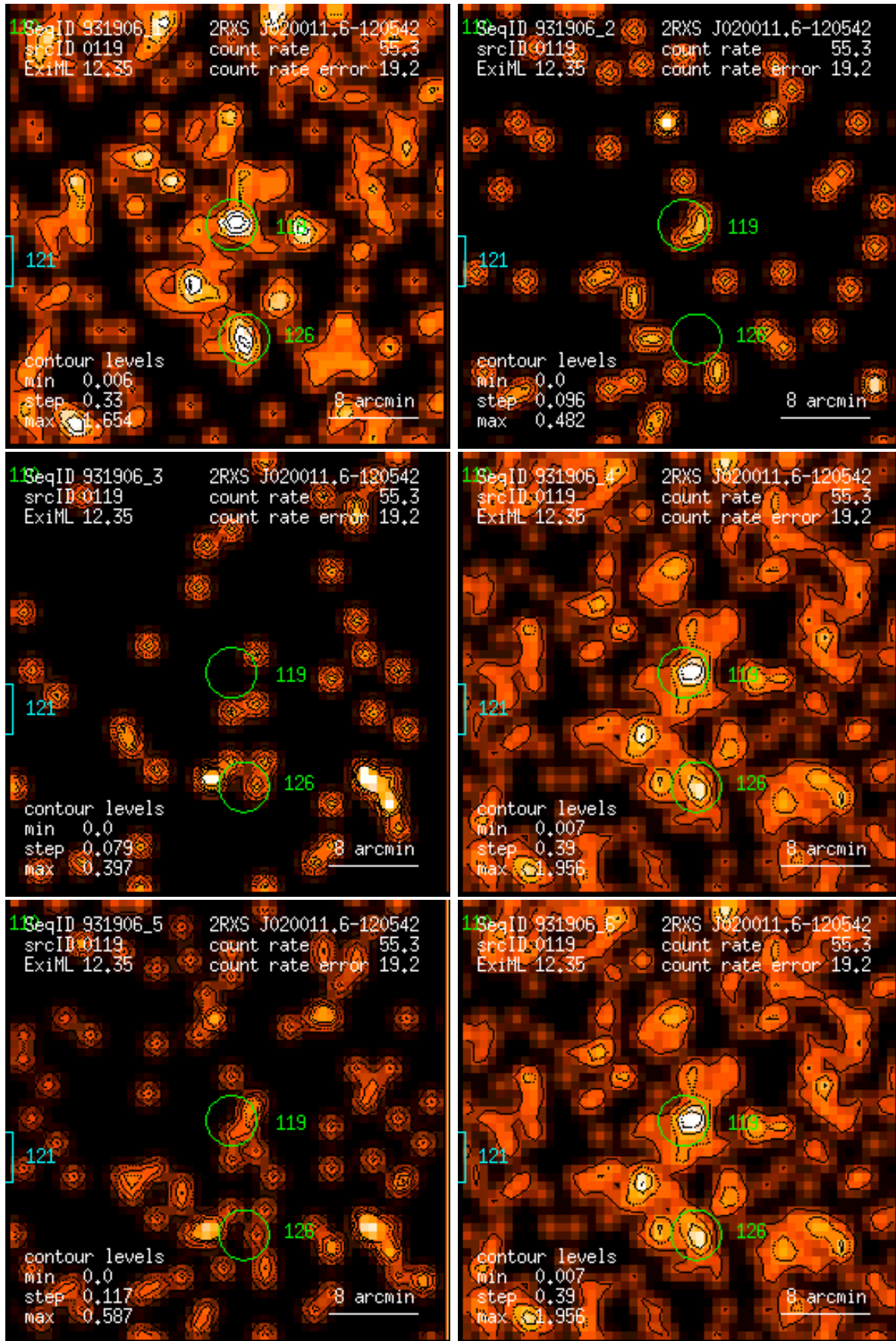
Figure 119: RASS 931906: detection 0119: band rate images, Gaussian filter: (1) PSPC channels 11 – 41, (2) 52 – 90, (3) 91 – 201, (4) 11 – 235, (5) 52 – 201, (6) 11 – 201. Broad band rates in counts/ks. Band rate contour levels in counts/ks/arcmin 2 .
