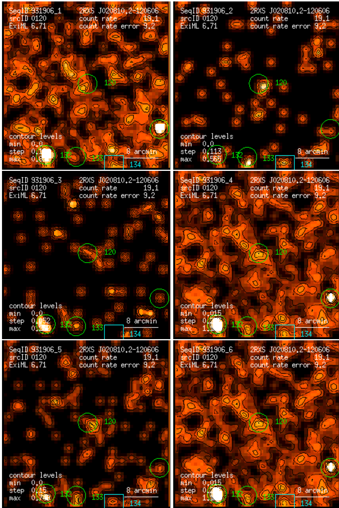
Figure 120: RASS 931906: detection 0120: band rate images, Gaussian filter: (1) PSPC channels 11 – 41, (2) 52 – 90, (3) 91 – 201, (4) 11 – 235, (5) 52 – 201, (6) 11 – 201. Broad band rates in counts/ks. Band rate contour levels in counts/ks/arcmin 2 .
