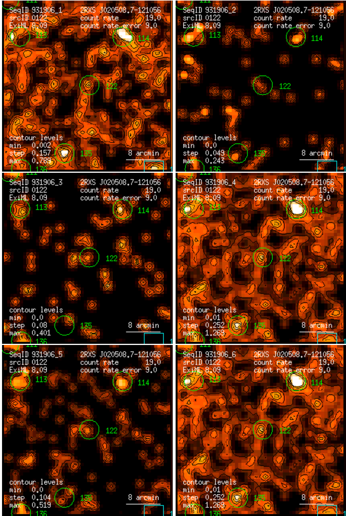
Figure 122: RASS 931906: detection 0122: band rate images, Gaussian filter: (1) PSPC channels 11 – 41, (2) 52 – 90, (3) 91 – 201, (4) 11 – 235, (5) 52 – 201, (6) 11 – 201. Broad band rates in counts/ks. Band rate contour levels in counts/ks/arcmin 2 .
