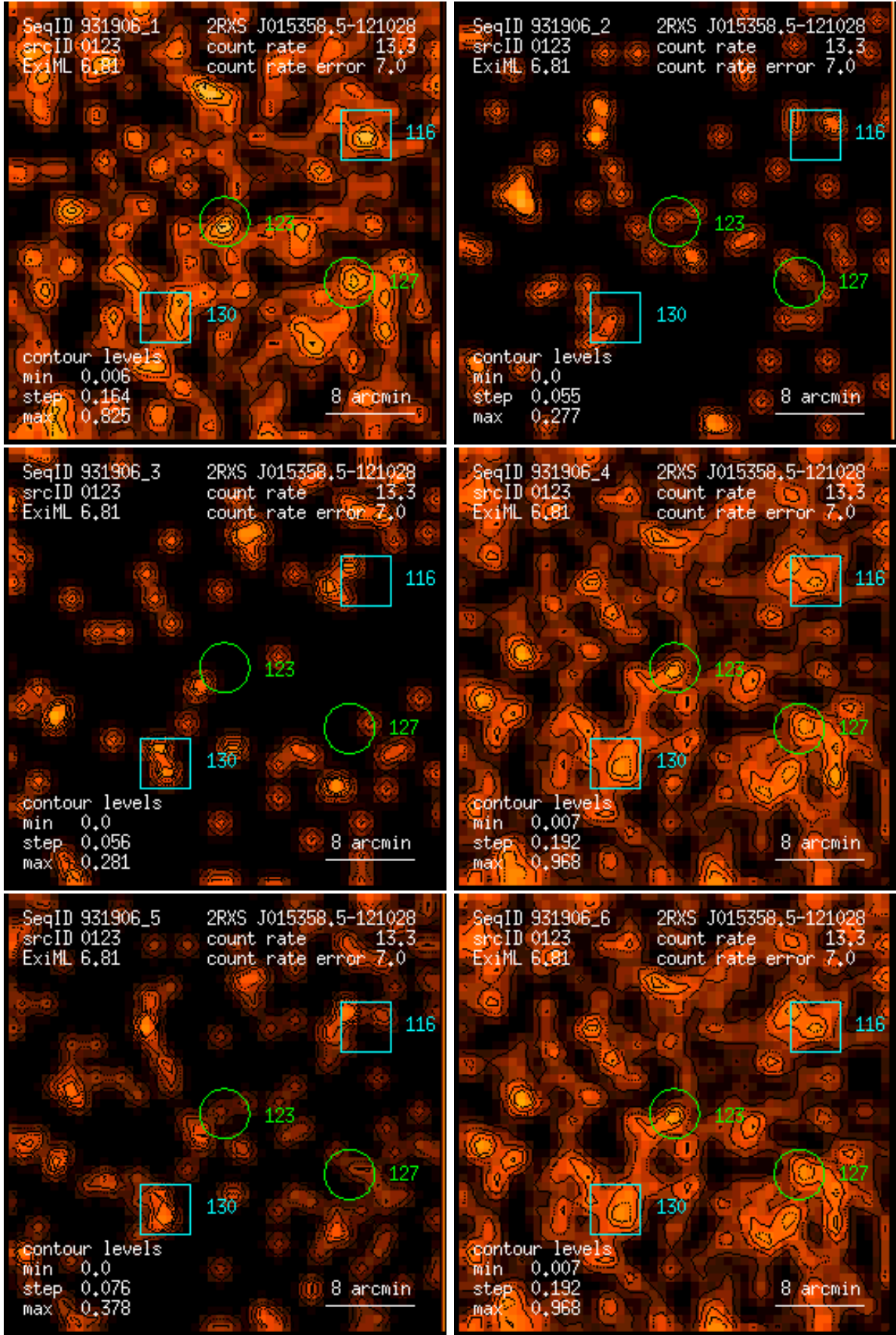
Figure 123: RASS 931906: detection 0123: band rate images, Gaussian filter: (1) PSPC channels 11 – 41, (2) 52 – 90, (3) 91 – 201, (4) 11 – 235, (5) 52 – 201, (6) 11 – 201. Broad band rates in counts/ks. Band rate contour levels in counts/ks/arcmin 2 .
