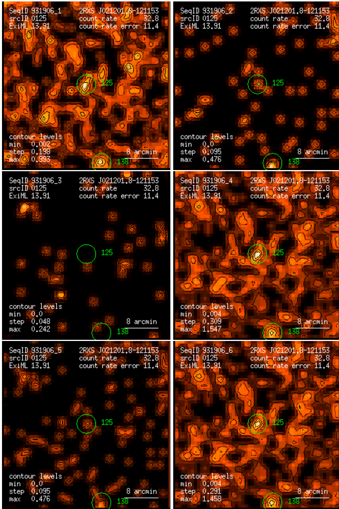
Figure 125: RASS 931906: detection 0125: band rate images, Gaussian filter: (1) PSPC channels 11 – 41, (2) 52 – 90, (3) 91 – 201, (4) 11 – 235, (5) 52 – 201, (6) 11 – 201. Broad band rates in counts/ks. Band rate contour levels in counts/ks/arcmin 2 .
