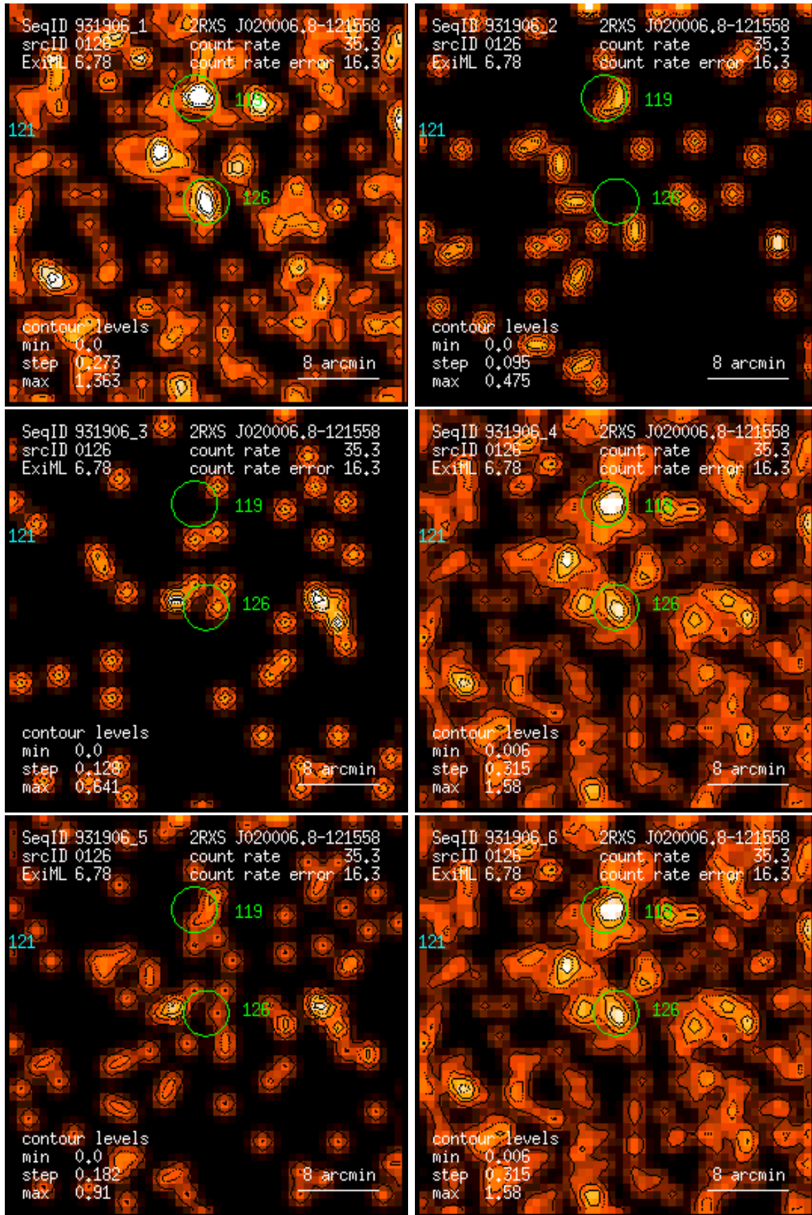
Figure 126: RASS 931906: detection 0126: band rate images, Gaussian filter: (1) PSPC channels 11 – 41, (2) 52 – 90, (3) 91 – 201, (4) 11 – 235, (5) 52 – 201, (6) 11 – 201. Broad band rates in counts/ks. Band rate contour levels in counts/ks/arcmin 2 .
