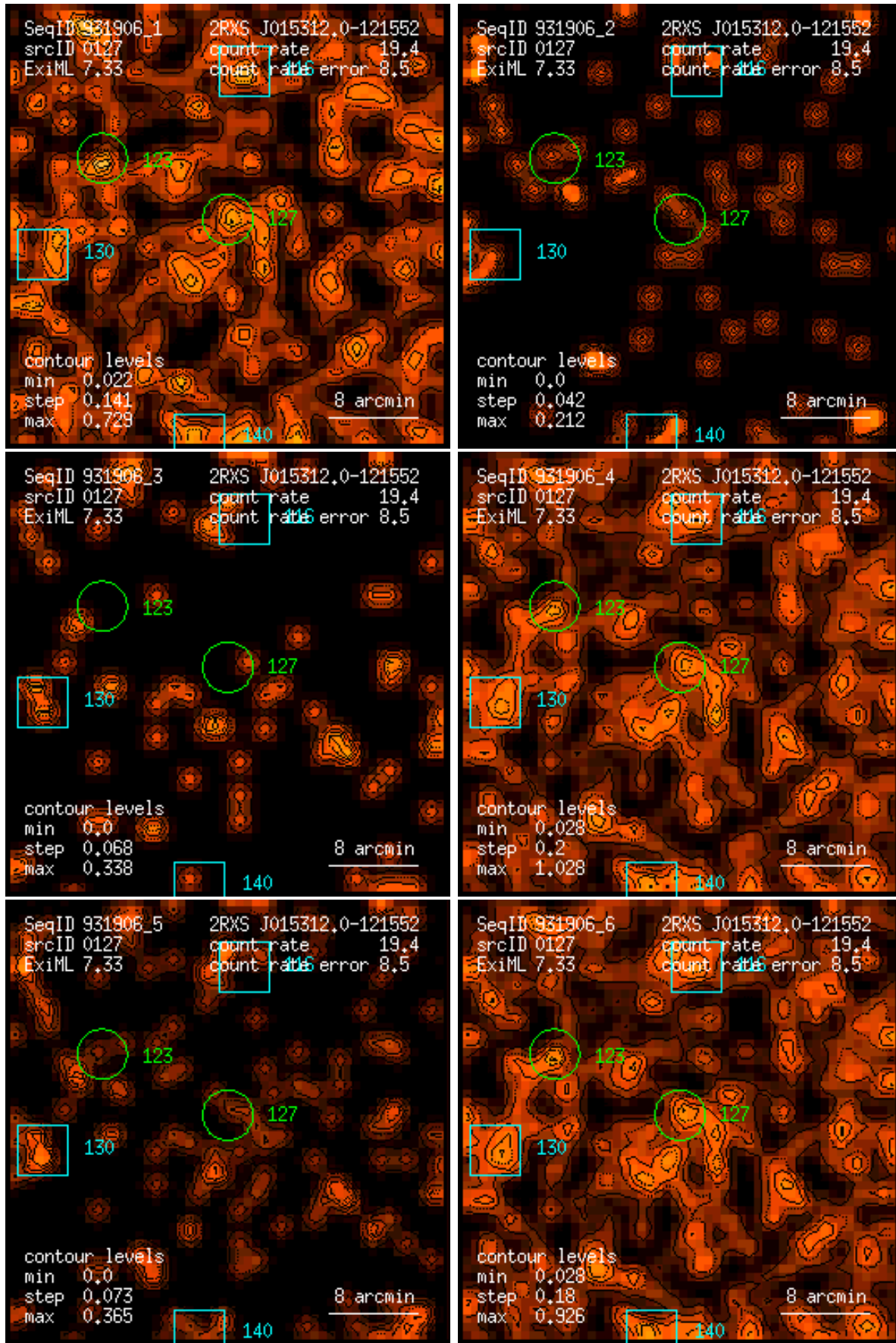
Figure 127: RASS 931906: detection 0127: band rate images, Gaussian filter: (1) PSPC channels 11 – 41, (2) 52 – 90, (3) 91 – 201, (4) 11 – 235, (5) 52 – 201, (6) 11 – 201. Broad band rates in counts/ks. Band rate contour levels in counts/ks/arcmin 2 .
