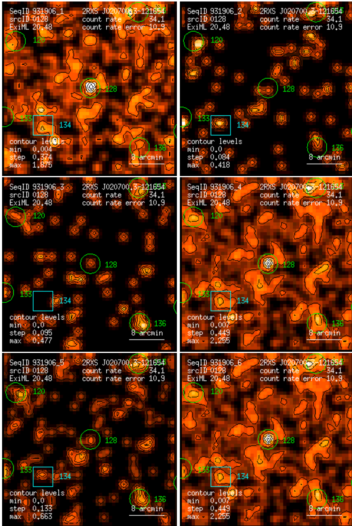
Figure 128: RASS 931906: detection 0128: band rate images, Gaussian filter: (1) PSPC channels 11 – 41, (2) 52 – 90, (3) 91 – 201, (4) 11 – 235, (5) 52 – 201, (6) 11 – 201. Broad band rates in counts/ks. Band rate contour levels in counts/ks/arcmin 2 .
