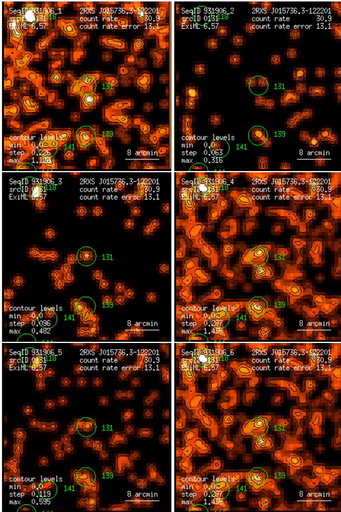
Figure 131: RASS 931906: detection 0131: band rate images, Gaussian filter: (1) PSPC channels 11 – 41, (2) 52 – 90, (3) 91 – 201, (4) 11 – 235, (5) 52 – 201, (6) 11 – 201. Broad band rates in counts/ks. Band rate contour levels in counts/ks/arcmin 2 .
