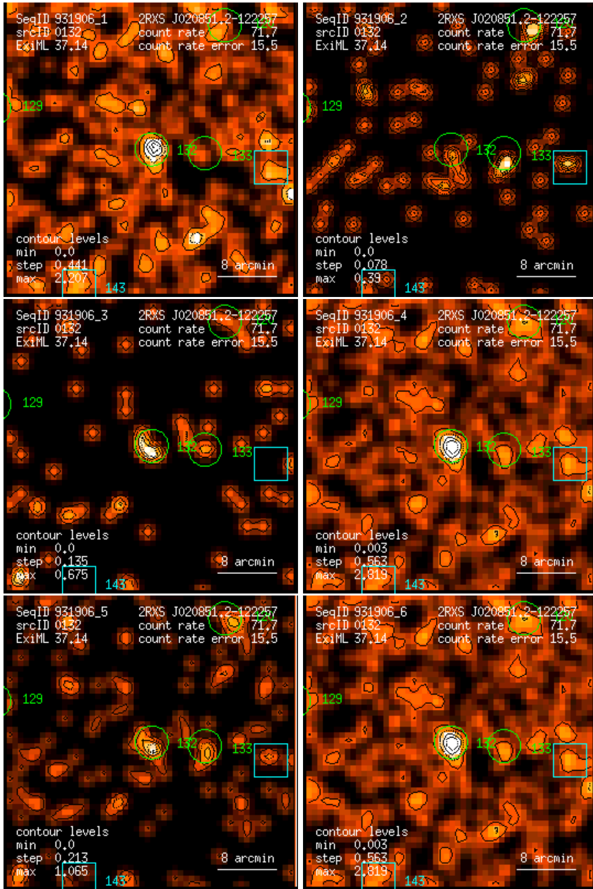
Figure 132: RASS 931906: detection 0132: band rate images, Gaussian filter: (1) PSPC channels 11 – 41, (2) 52 – 90, (3) 91 – 201, (4) 11 – 235, (5) 52 – 201, (6) 11 – 201. Broad band rates in counts/ks. Band rate contour levels in counts/ks/arcmin 2 .
