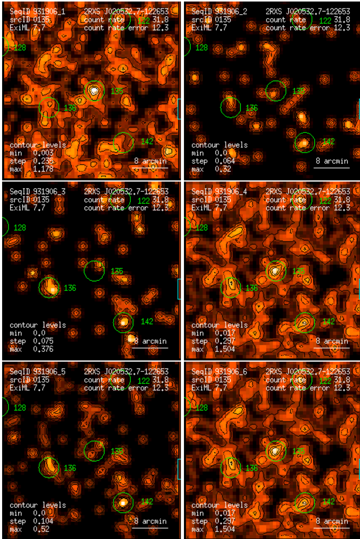
Figure 135: RASS 931906: detection 0135: band rate images, Gaussian filter: (1) PSPC channels 11 – 41, (2) 52 – 90, (3) 91 – 201, (4) 11 – 235, (5) 52 – 201, (6) 11 – 201. Broad band rates in counts/ks. Band rate contour levels in counts/ks/arcmin 2 .
