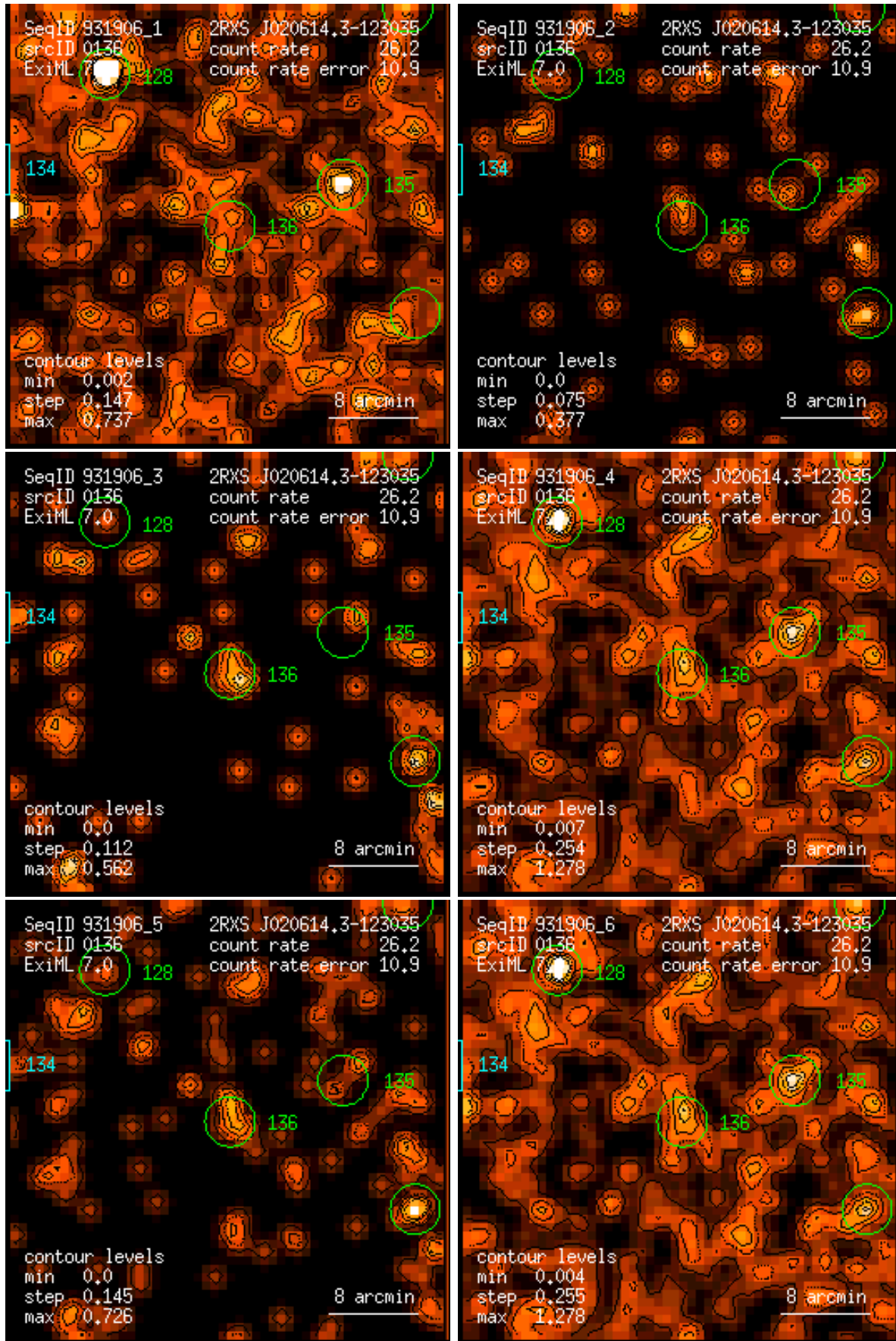
Figure 136: RASS 931906: detection 0136: band rate images, Gaussian filter: (1) PSPC channels 11 – 41, (2) 52 – 90, (3) 91 – 201, (4) 11 – 235, (5) 52 – 201, (6) 11 – 201. Broad band rates in counts/ks. Band rate contour levels in counts/ks/arcmin 2 .
