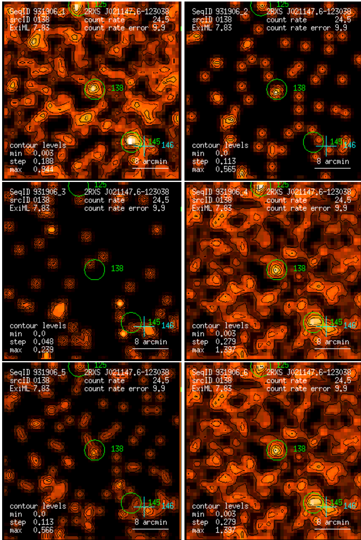
Figure 138: RASS 931906: detection 0138: band rate images, Gaussian filter: (1) PSPC channels 11 – 41, (2) 52 – 90, (3) 91 – 201, (4) 11 – 235, (5) 52 – 201, (6) 11 – 201. Broad band rates in counts/ks. Band rate contour levels in counts/ks/arcmin 2 .
