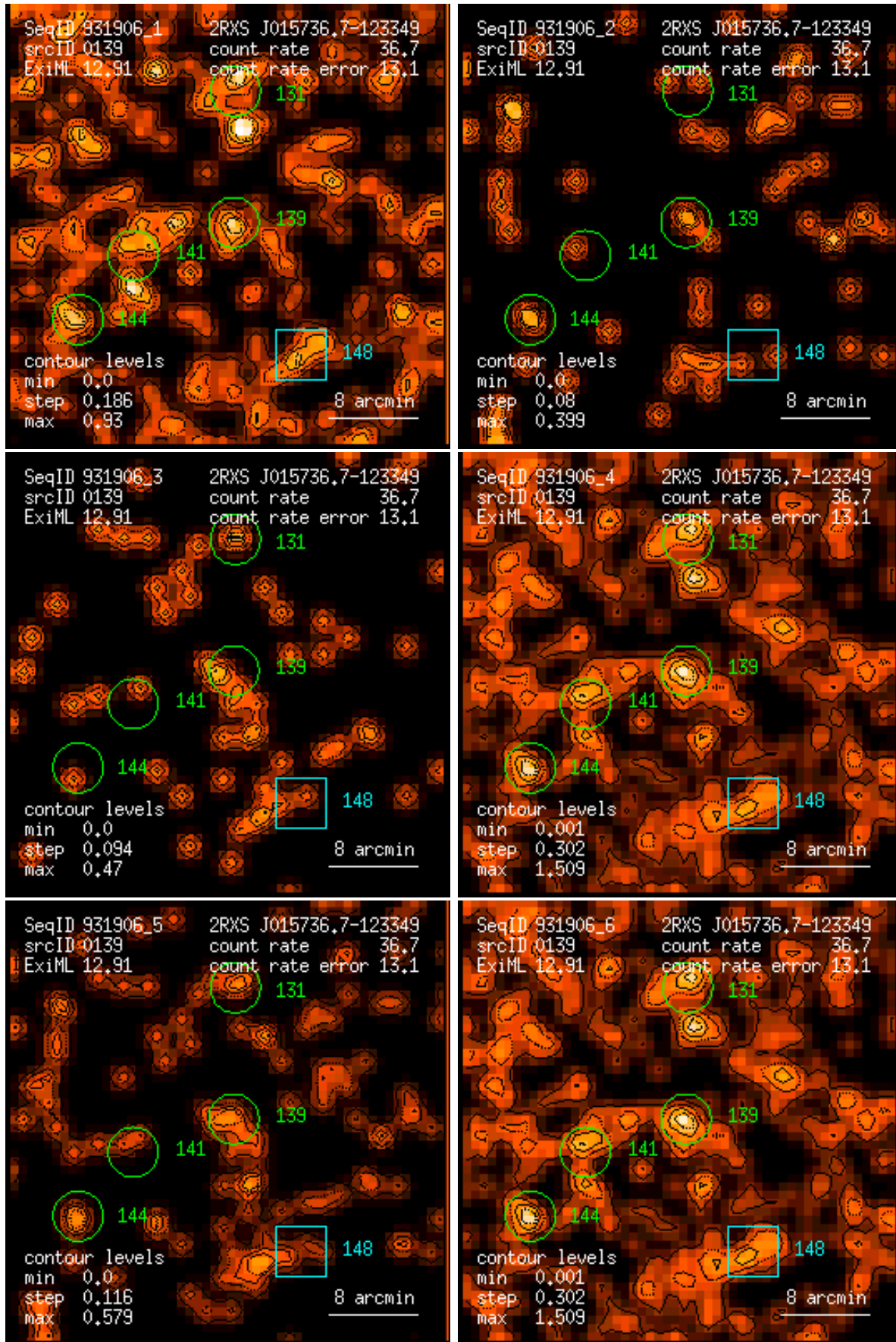
Figure 139: RASS 931906: detection 0139: band rate images, Gaussian filter: (1) PSPC channels 11 – 41, (2) 52 – 90, (3) 91 – 201, (4) 11 – 235, (5) 52 – 201, (6) 11 – 201. Broad band rates in counts/ks. Band rate contour levels in counts/ks/arcmin 2 .
