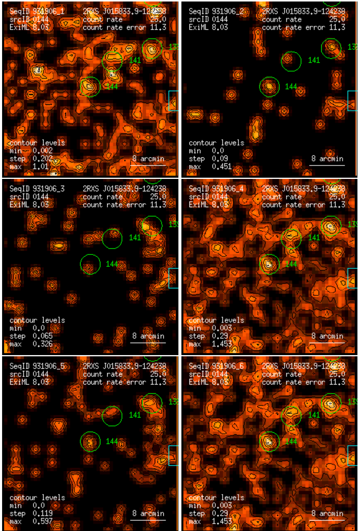
Figure 144: RASS 931906: detection 0144: band rate images, Gaussian filter: (1) PSPC channels 11 – 41, (2) 52 – 90, (3) 91 – 201, (4) 11 – 235, (5) 52 – 201, (6) 11 – 201. Broad band rates in counts/ks. Band rate contour levels in counts/ks/arcmin 2 .
