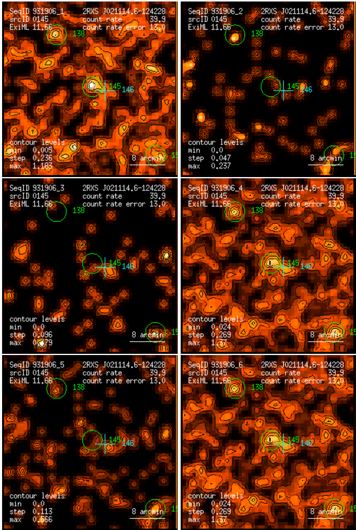
Figure 145: RASS 931906: detection 0145: band rate images, Gaussian filter: (1) PSPC channels 11 – 41, (2) 52 – 90, (3) 91 – 201, (4) 11 – 235, (5) 52 – 201, (6) 11 – 201. Broad band rates in counts/ks. Band rate contour levels in counts/ks/arcmin 2 .
