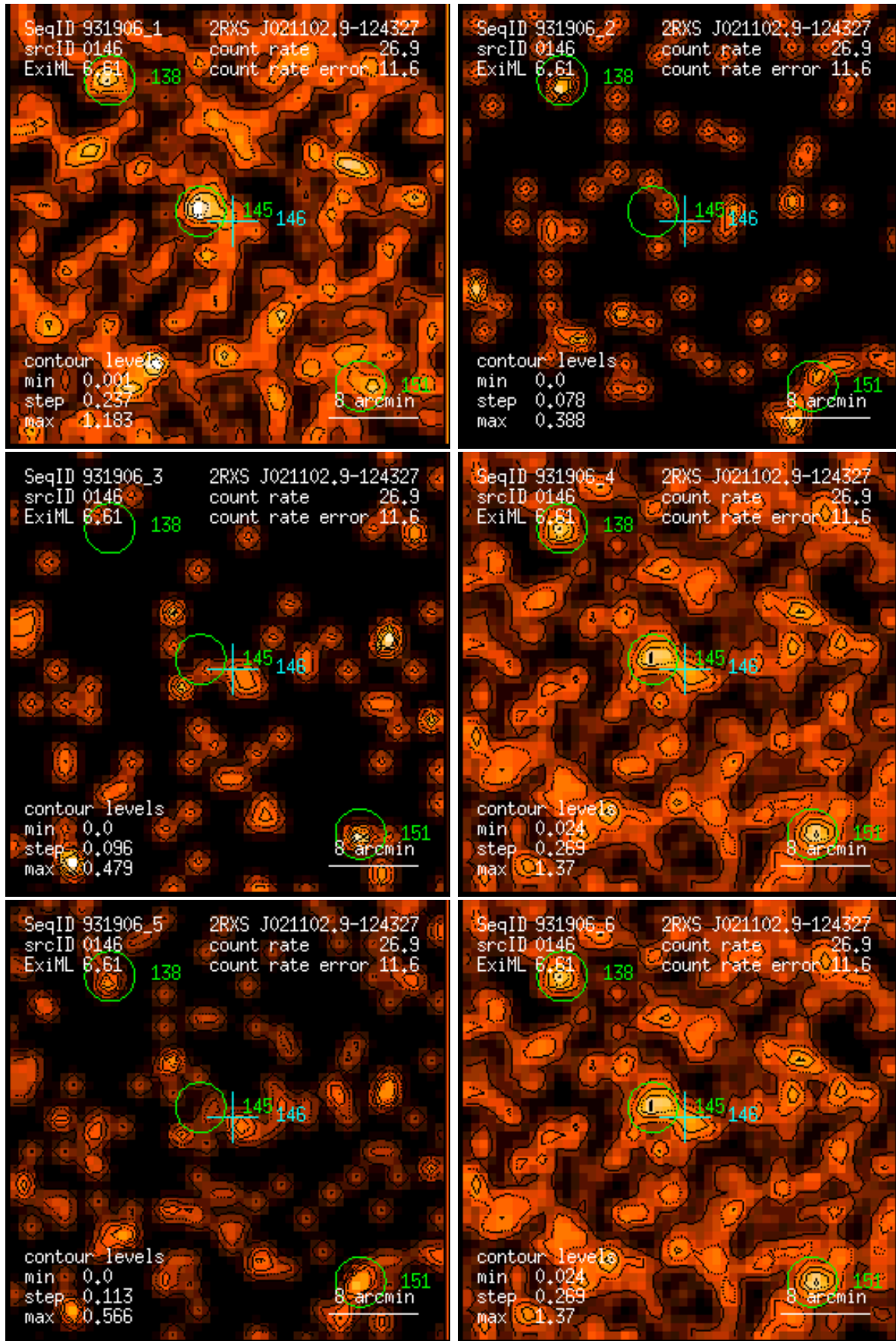
Figure 146: RASS 931906: detection 0146: band rate images, Gaussian filter: (1) PSPC channels 11 – 41, (2) 52 – 90, (3) 91 – 201, (4) 11 – 235, (5) 52 – 201, (6) 11 – 201. Broad band rates in counts/ks. Band rate contour levels in counts/ks/arcmin 2 .
