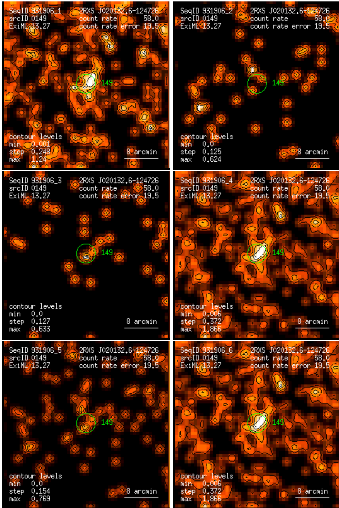
Figure 149: RASS 931906: detection 0149: band rate images, Gaussian filter: (1) PSPC channels 11 – 41, (2) 52 – 90, (3) 91 – 201, (4) 11 – 235, (5) 52 – 201, (6) 11 – 201. Broad band rates in counts/ks. Band rate contour levels in counts/ks/arcmin 2 .
