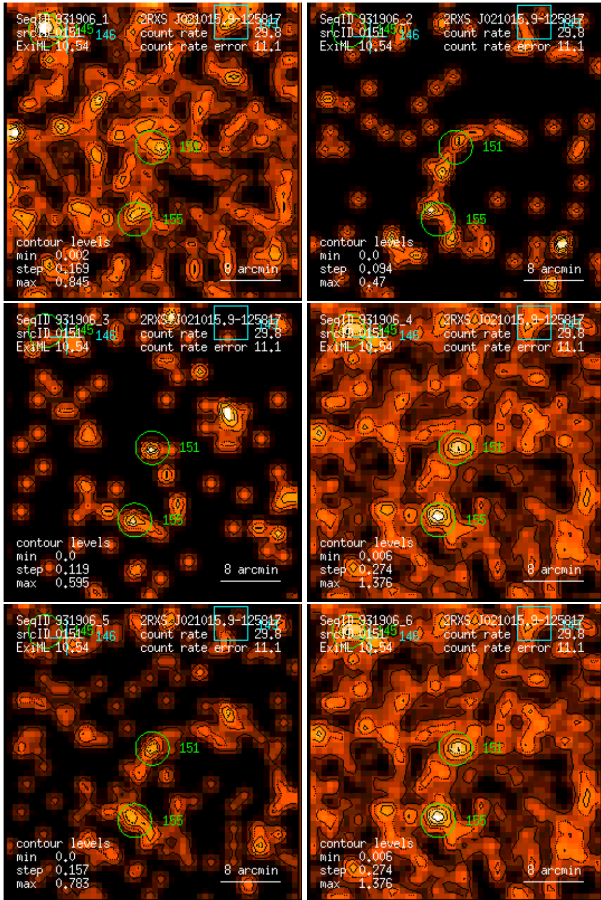
Figure 151: RASS 931906: detection 0151: band rate images, Gaussian filter: (1) PSPC channels 11 – 41, (2) 52 – 90, (3) 91 – 201, (4) 11 – 235, (5) 52 – 201, (6) 11 – 201. Broad band rates in counts/ks. Band rate contour levels in counts/ks/arcmin 2 .
