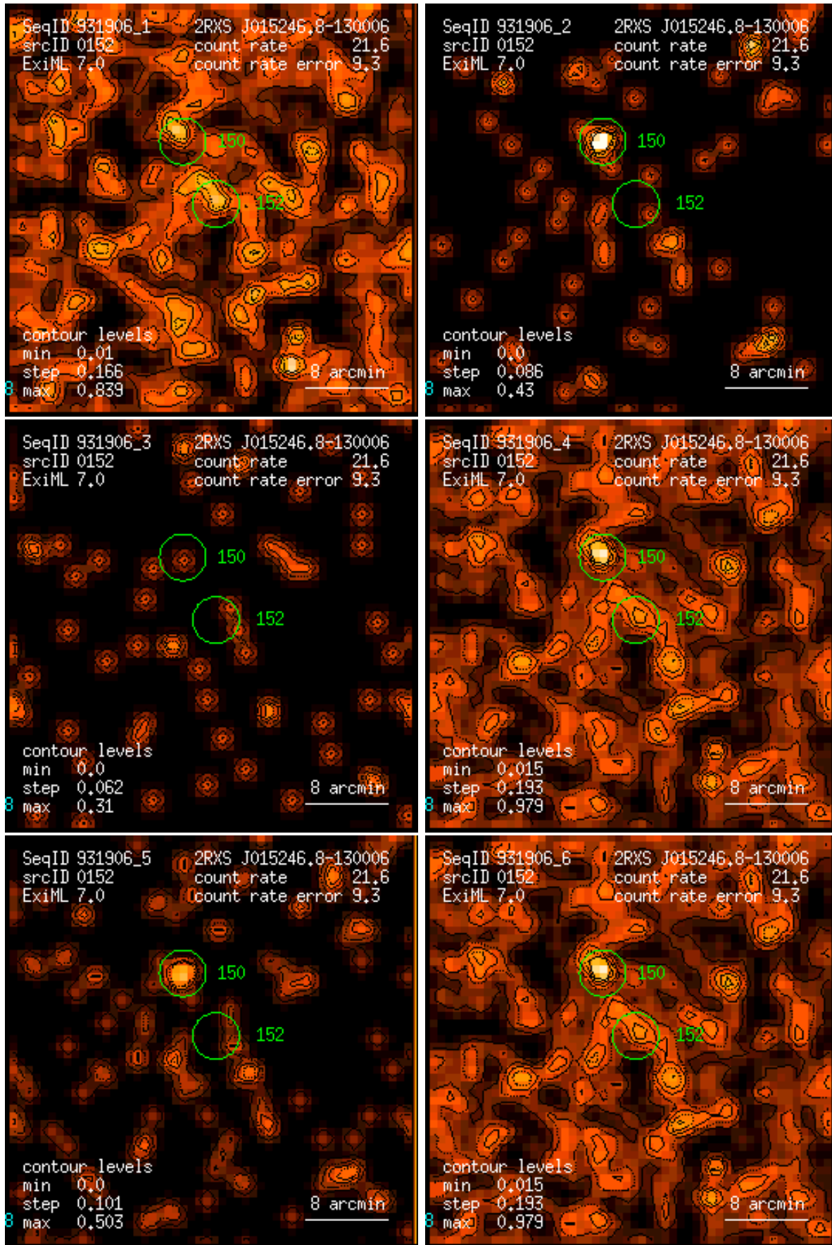
Figure 152: RASS 931906: detection 0152: band rate images, Gaussian filter: (1) PSPC channels 11 – 41, (2) 52 – 90, (3) 91 – 201, (4) 11 – 235, (5) 52 – 201, (6) 11 – 201. Broad band rates in counts/ks. Band rate contour levels in counts/ks/arcmin 2 .
