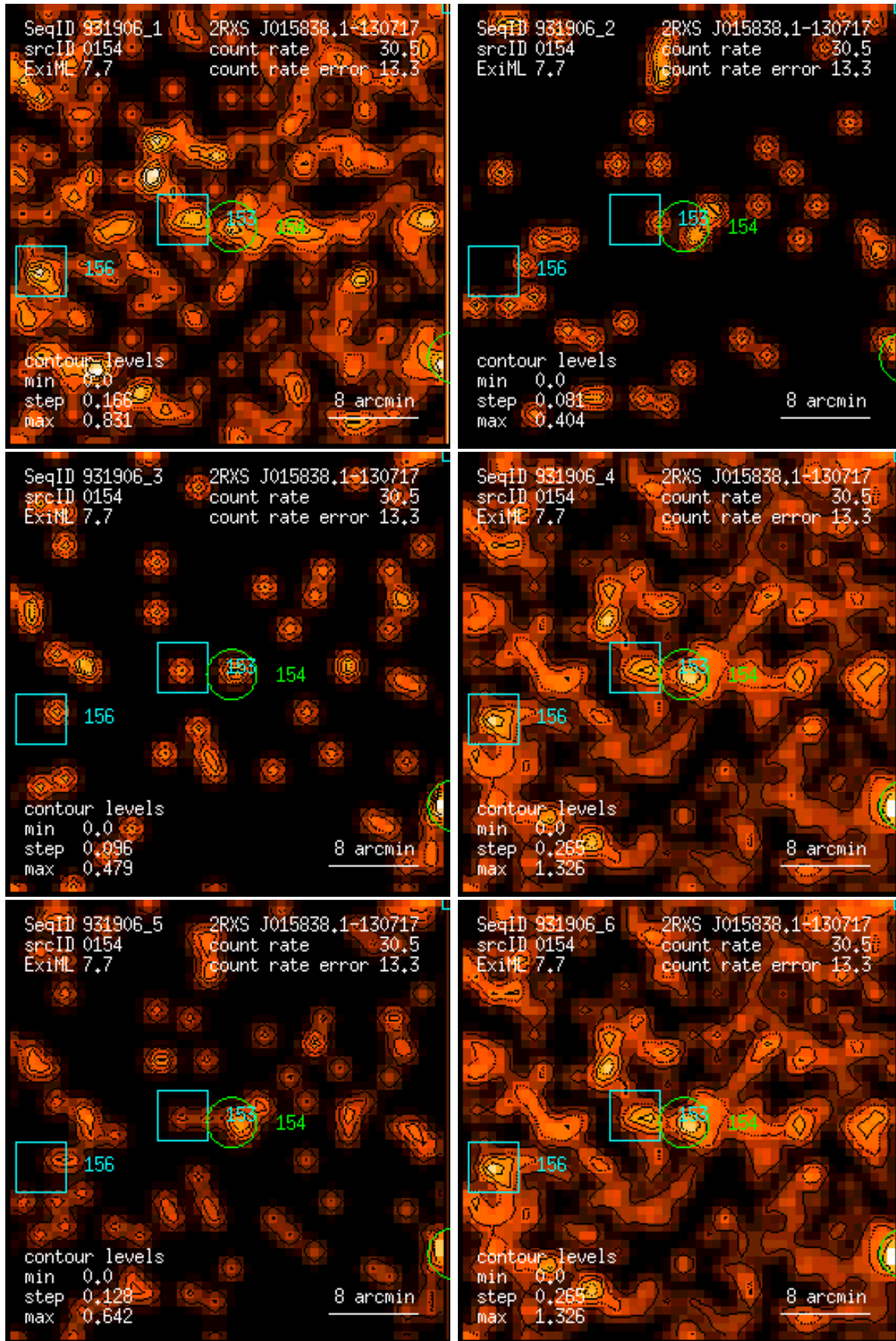
Figure 154: RASS 931906: detection 0154: band rate images, Gaussian filter: (1) PSPC channels 11 – 41, (2) 52 – 90, (3) 91 – 201, (4) 11 – 235, (5) 52 – 201, (6) 11 – 201. Broad band rates in counts/ks. Band rate contour levels in counts/ks/arcmin 2 .
