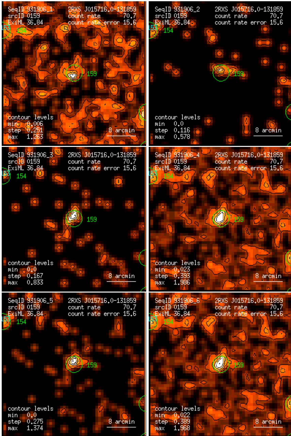
Figure 159: RASS 931906: detection 0159: band rate images, Gaussian filter: (1) PSPC channels 11 – 41, (2) 52 – 90, (3) 91 – 201, (4) 11 – 235, (5) 52 – 201, (6) 11 – 201. Broad band rates in counts/ks. Band rate contour levels in counts/ks/arcmin 2 .
