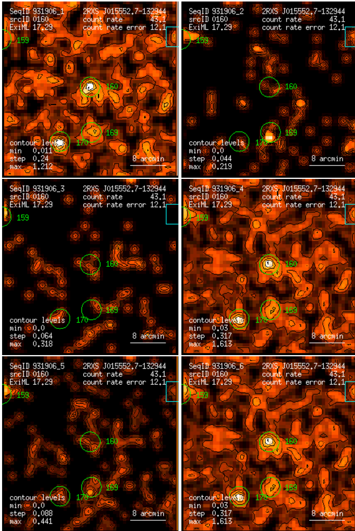
Figure 160: RASS 931906: detection 0160: band rate images, Gaussian filter: (1) PSPC channels 11 – 41, (2) 52 – 90, (3) 91 – 201, (4) 11 – 235, (5) 52 – 201, (6) 11 – 201. Broad band rates in counts/ks. Band rate contour levels in counts/ks/arcmin 2 .
