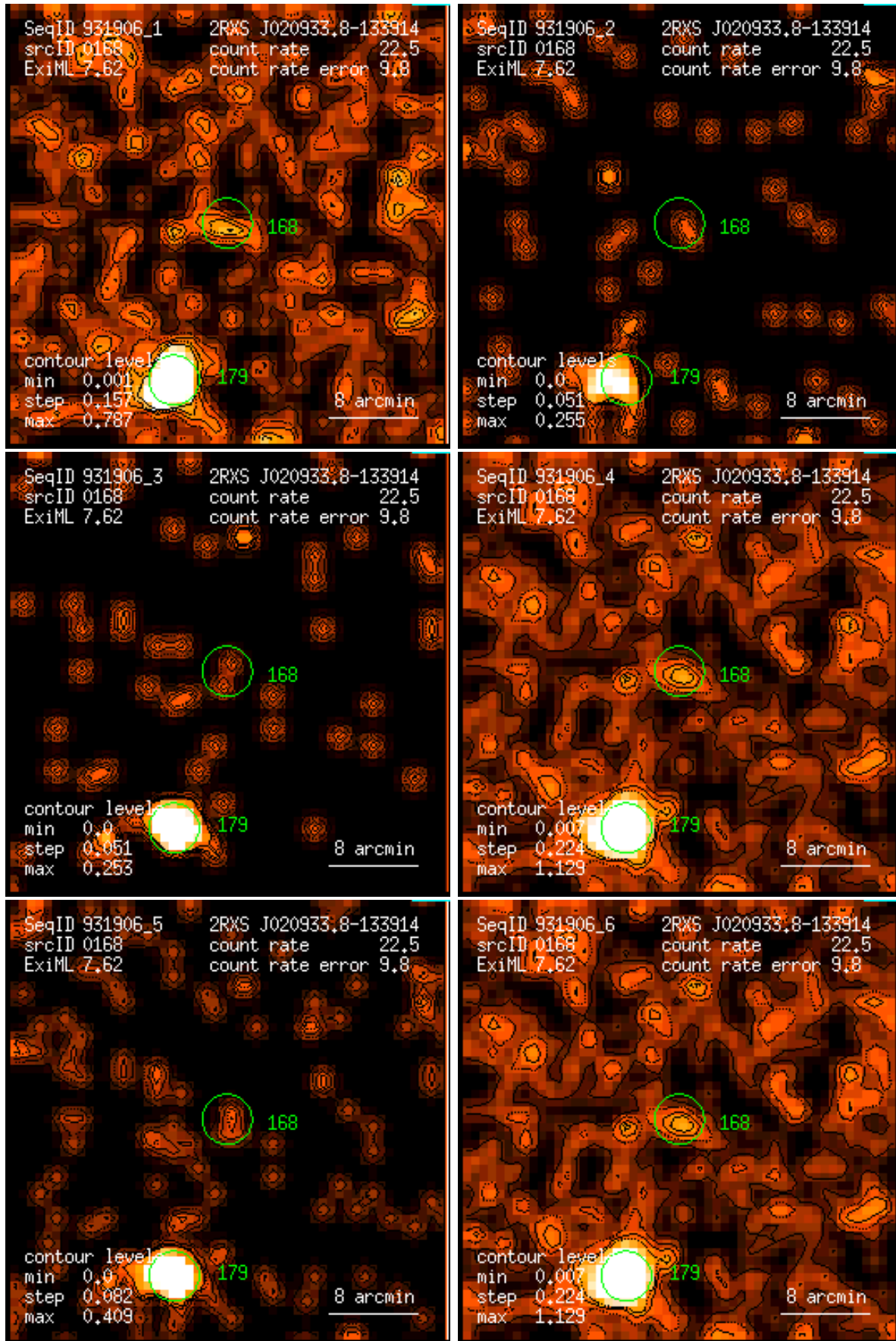
Figure 168: RASS 931906: detection 0168: band rate images, Gaussian filter: (1) PSPC channels 11 – 41, (2) 52 – 90, (3) 91 – 201, (4) 11 – 235, (5) 52 – 201, (6) 11 – 201. Broad band rates in counts/ks. Band rate contour levels in counts/ks/arcmin 2 .
