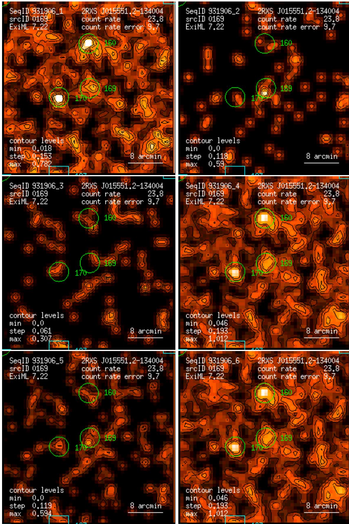
Figure 169: RASS 931906: detection 0169: band rate images, Gaussian filter: (1) PSPC channels 11 – 41, (2) 52 – 90, (3) 91 – 201, (4) 11 – 235, (5) 52 – 201, (6) 11 – 201. Broad band rates in counts/ks. Band rate contour levels in counts/ks/arcmin 2 .
