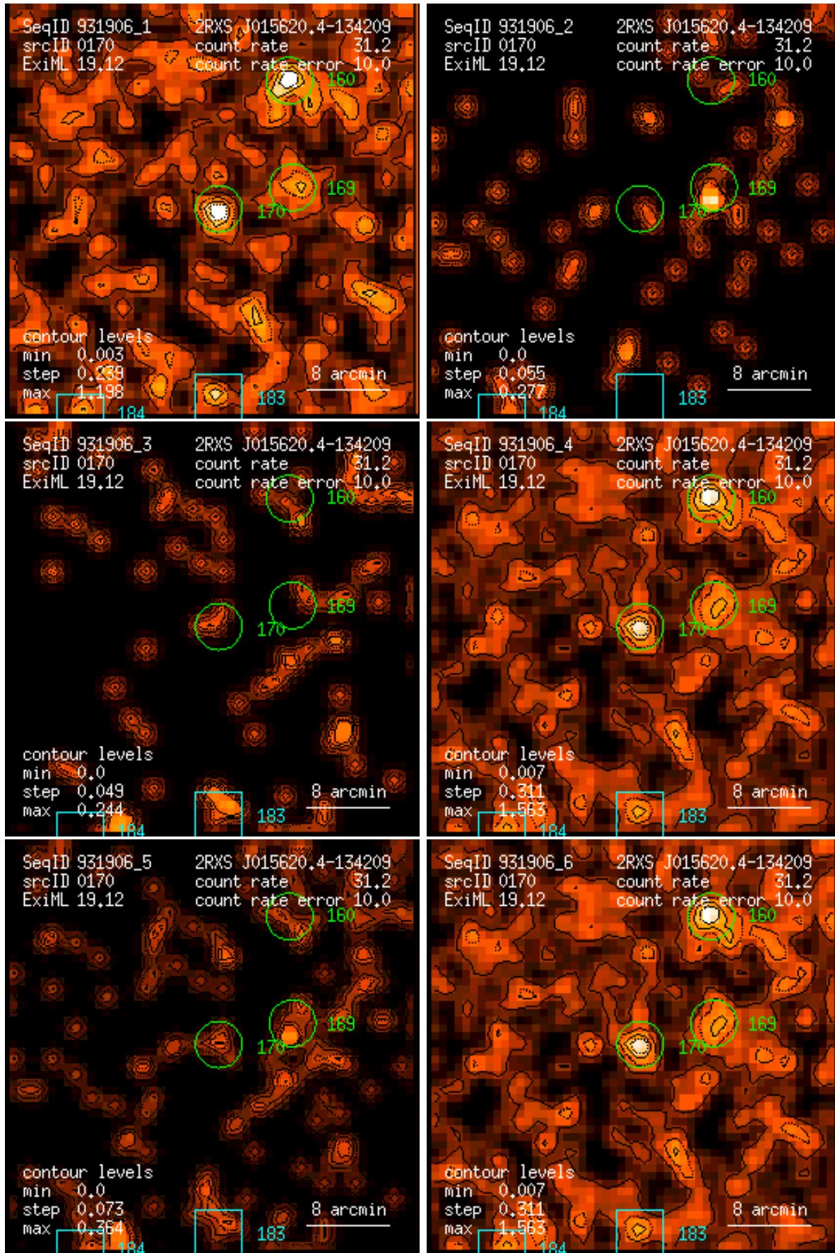
Figure 170: RASS 931906: detection 0170: band rate images, Gaussian filter: (1) PSPC channels 11 – 41, (2) 52 – 90, (3) 91 – 201, (4) 11 – 235, (5) 52 – 201, (6) 11 – 201. Broad band rates in counts/ks. Band rate contour levels in counts/ks/arcmin 2 .
