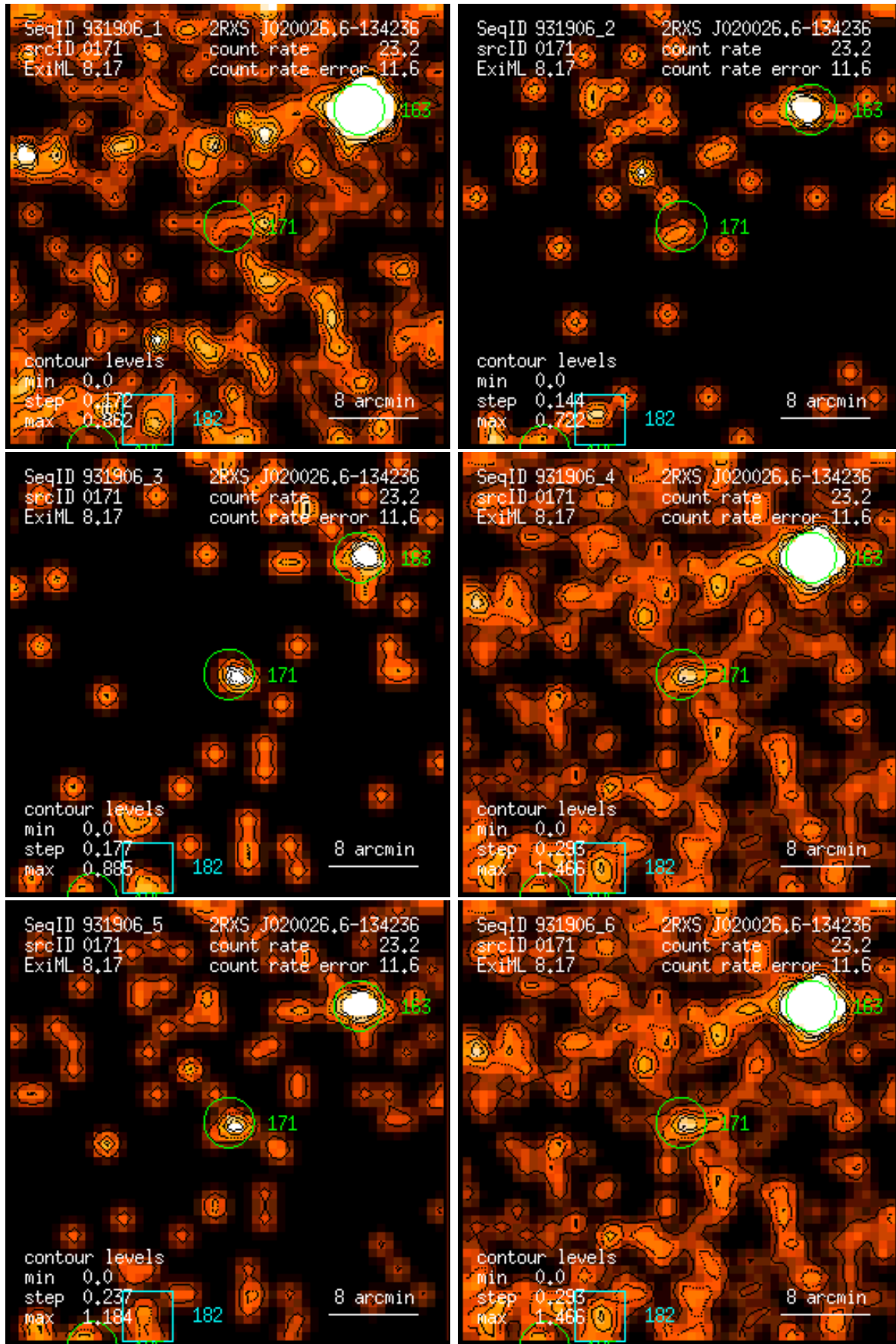
Figure 171: RASS 931906: detection 0171: band rate images, Gaussian filter: (1) PSPC channels 11 – 41, (2) 52 – 90, (3) 91 – 201, (4) 11 – 235, (5) 52 – 201, (6) 11 – 201. Broad band rates in counts/ks. Band rate contour levels in counts/ks/arcmin 2 .
