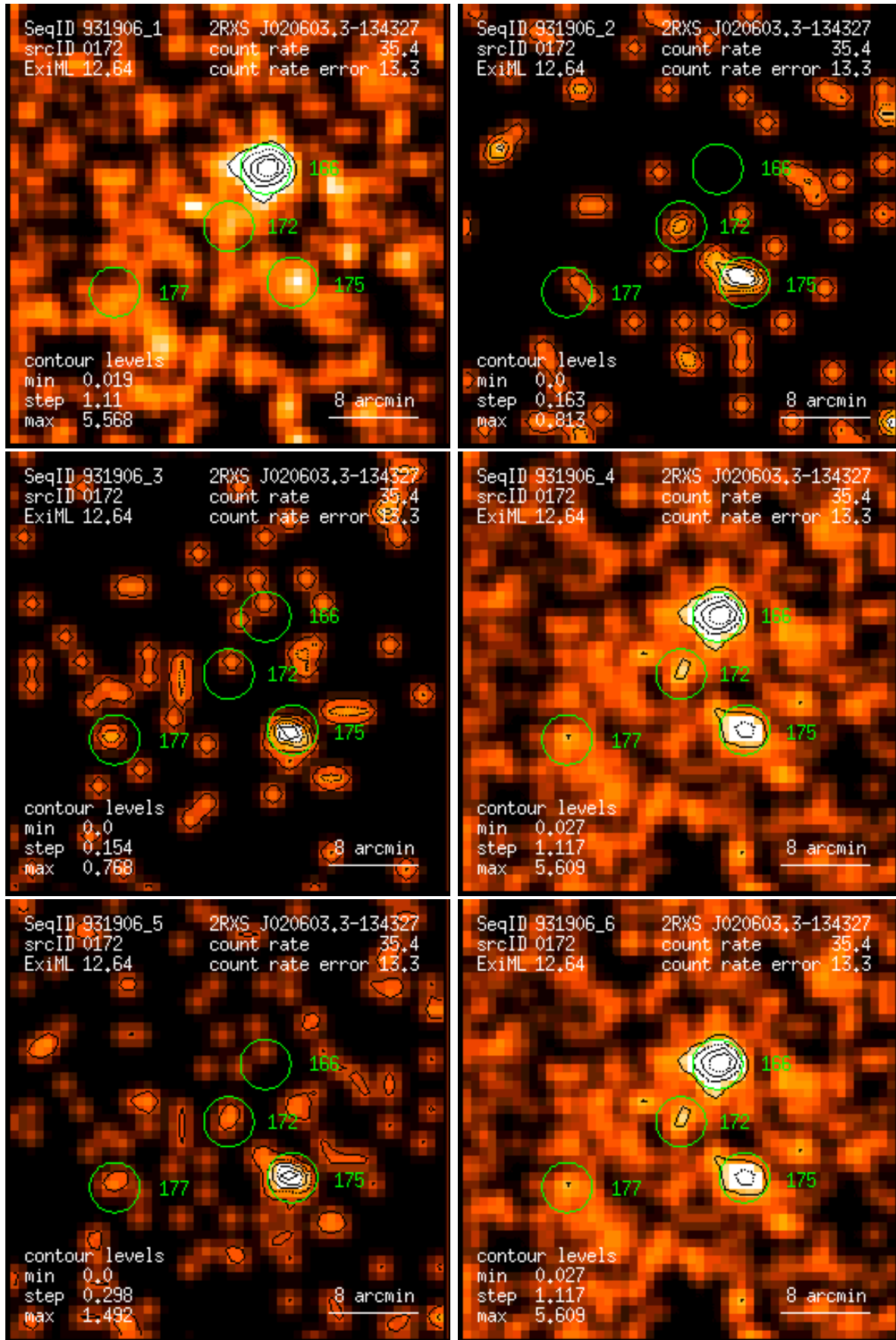
Figure 172: RASS 931906: detection 0172: band rate images, Gaussian filter: (1) PSPC channels 11 – 41, (2) 52 – 90, (3) 91 – 201, (4) 11 – 235, (5) 52 – 201, (6) 11 – 201. Broad band rates in counts/ks. Band rate contour levels in counts/ks/arcmin 2 .
