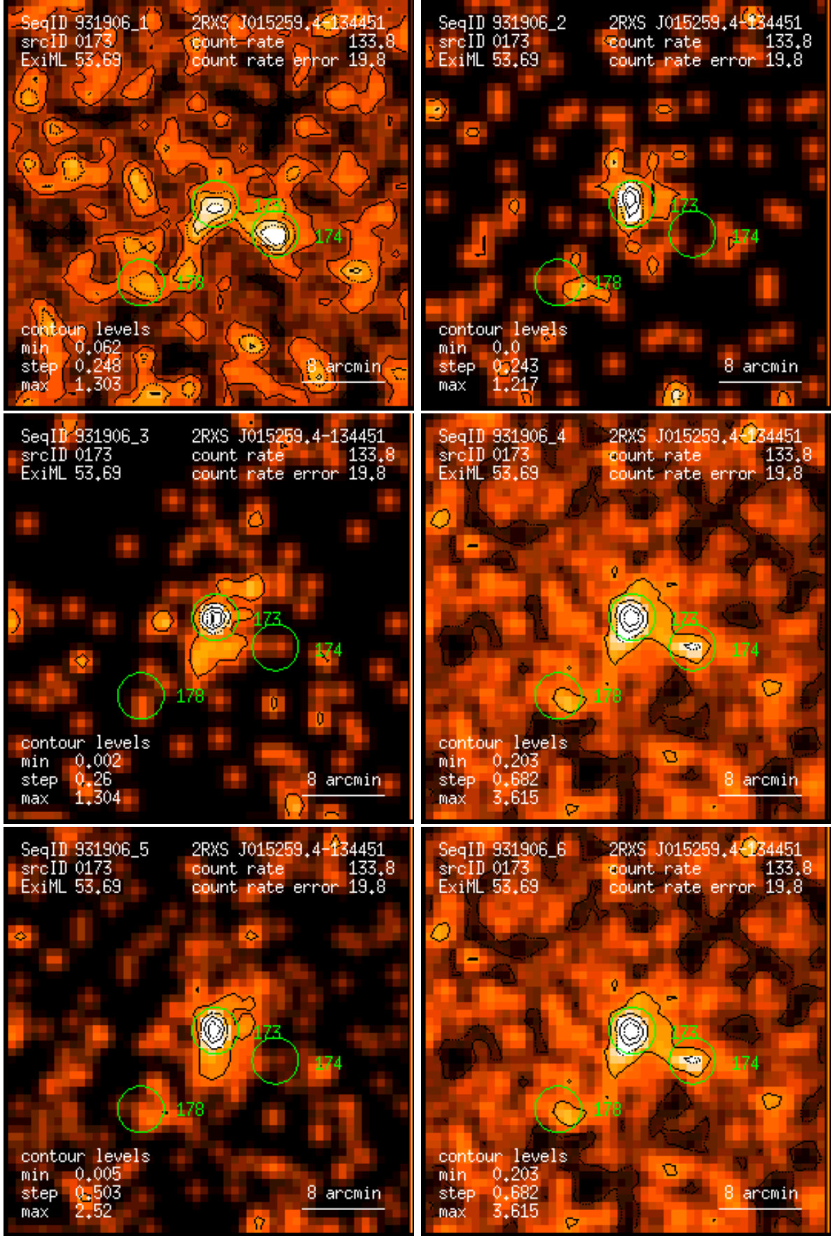
Figure 173: RASS 931906: detection 0173: band rate images, Gaussian filter: (1) PSPC channels 11 – 41, (2) 52 – 90, (3) 91 – 201, (4) 11 – 235, (5) 52 – 201, (6) 11 – 201. Broad band rates in counts/ks. Band rate contour levels in counts/ks/arcmin 2 .
