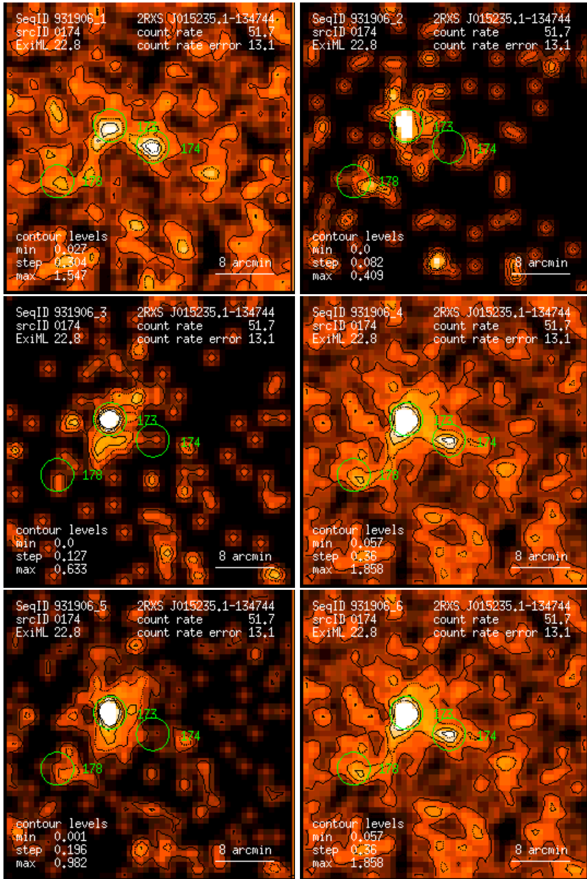
Figure 174: RASS 931906: detection 0174: band rate images, Gaussian filter: (1) PSPC channels 11 – 41, (2) 52 – 90, (3) 91 – 201, (4) 11 – 235, (5) 52 – 201, (6) 11 – 201. Broad band rates in counts/ks. Band rate contour levels in counts/ks/arcmin 2 .
