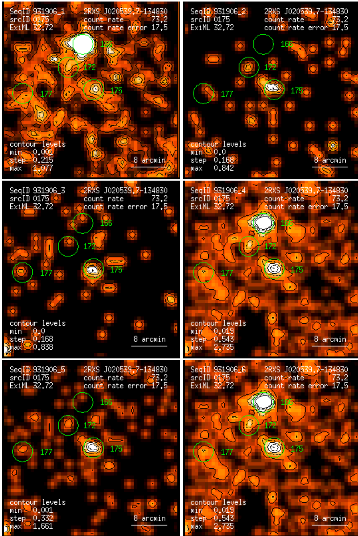
Figure 175: RASS 931906: detection 0175: band rate images, Gaussian filter: (1) PSPC channels 11 – 41, (2) 52 – 90, (3) 91 – 201, (4) 11 – 235, (5) 52 – 201, (6) 11 – 201. Broad band rates in counts/ks. Band rate contour levels in counts/ks/arcmin 2 .
