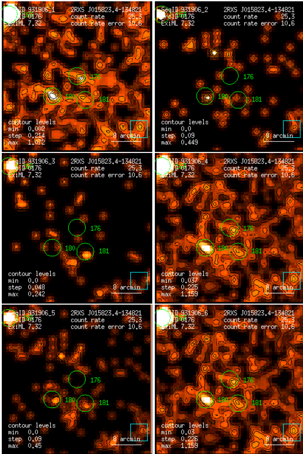
Figure 176: RASS 931906: detection 0176: band rate images, Gaussian filter: (1) PSPC channels 11 – 41, (2) 52 – 90, (3) 91 – 201, (4) 11 – 235, (5) 52 – 201, (6) 11 – 201. Broad band rates in counts/ks. Band rate contour levels in counts/ks/arcmin 2 .
