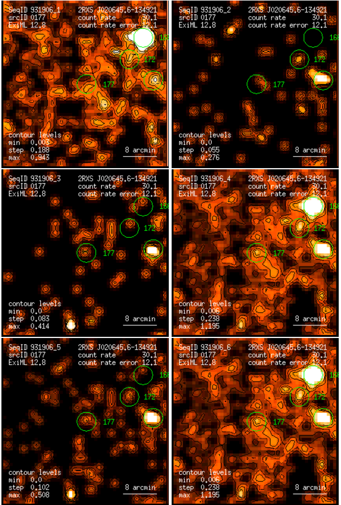
Figure 177: RASS 931906: detection 0177: band rate images, Gaussian filter: (1) PSPC channels 11 – 41, (2) 52 – 90, (3) 91 – 201, (4) 11 – 235, (5) 52 – 201, (6) 11 – 201. Broad band rates in counts/ks. Band rate contour levels in counts/ks/arcmin 2 .
