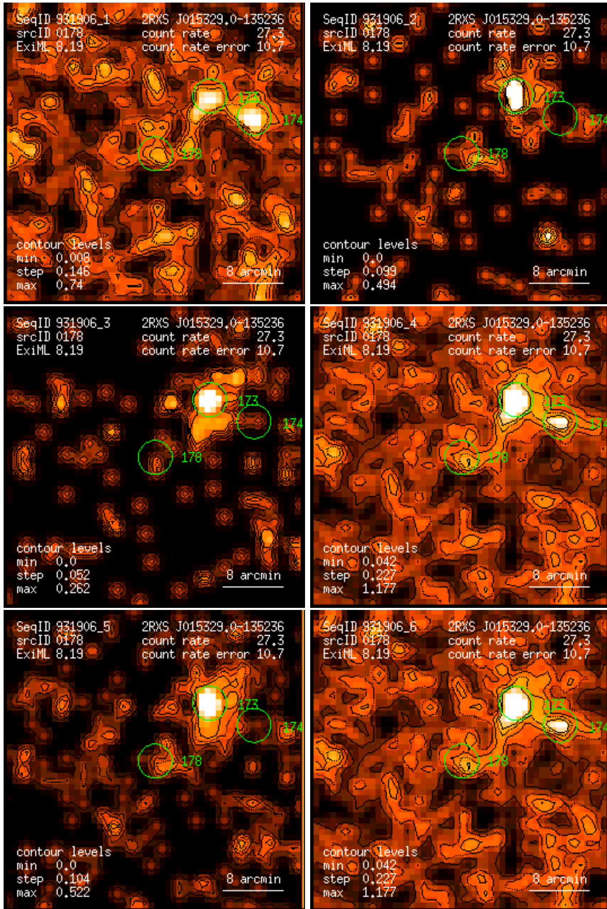
Figure 178: RASS 931906: detection 0178: band rate images, Gaussian filter: (1) PSPC channels 11 – 41, (2) 52 – 90, (3) 91 – 201, (4) 11 – 235, (5) 52 – 201, (6) 11 – 201. Broad band rates in counts/ks. Band rate contour levels in counts/ks/arcmin 2 .
