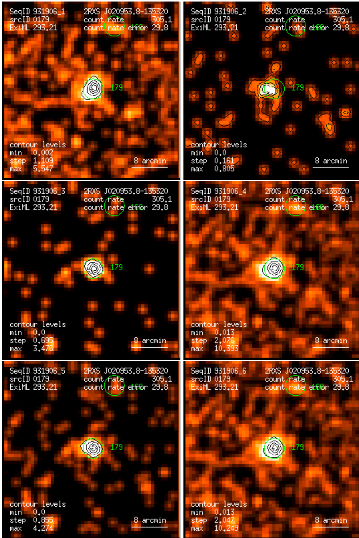
Figure 179: RASS 931906: detection 0179: band rate images, Gaussian filter: (1) PSPC channels 11 – 41, (2) 52 – 90, (3) 91 – 201, (4) 11 – 235, (5) 52 – 201, (6) 11 – 201. Broad band rates in counts/ks. Band rate contour levels in counts/ks/arcmin 2 .
