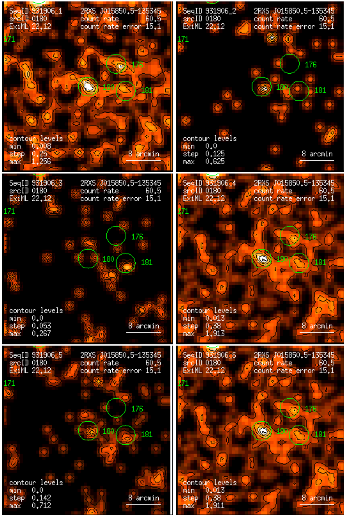
Figure 180: RASS 931906: detection 0180: band rate images, Gaussian filter: (1) PSPC channels 11 – 41, (2) 52 – 90, (3) 91 – 201, (4) 11 – 235, (5) 52 – 201, (6) 11 – 201. Broad band rates in counts/ks. Band rate contour levels in counts/ks/arcmin 2 .
