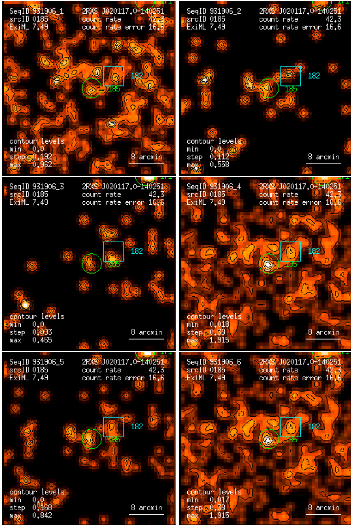
Figure 185: RASS 931906: detection 0185: band rate images, Gaussian filter: (1) PSPC channels 11 – 41, (2) 52 – 90, (3) 91 – 201, (4) 11 – 235, (5) 52 – 201, (6) 11 – 201. Broad band rates in counts/ks. Band rate contour levels in counts/ks/arcmin 2 .
