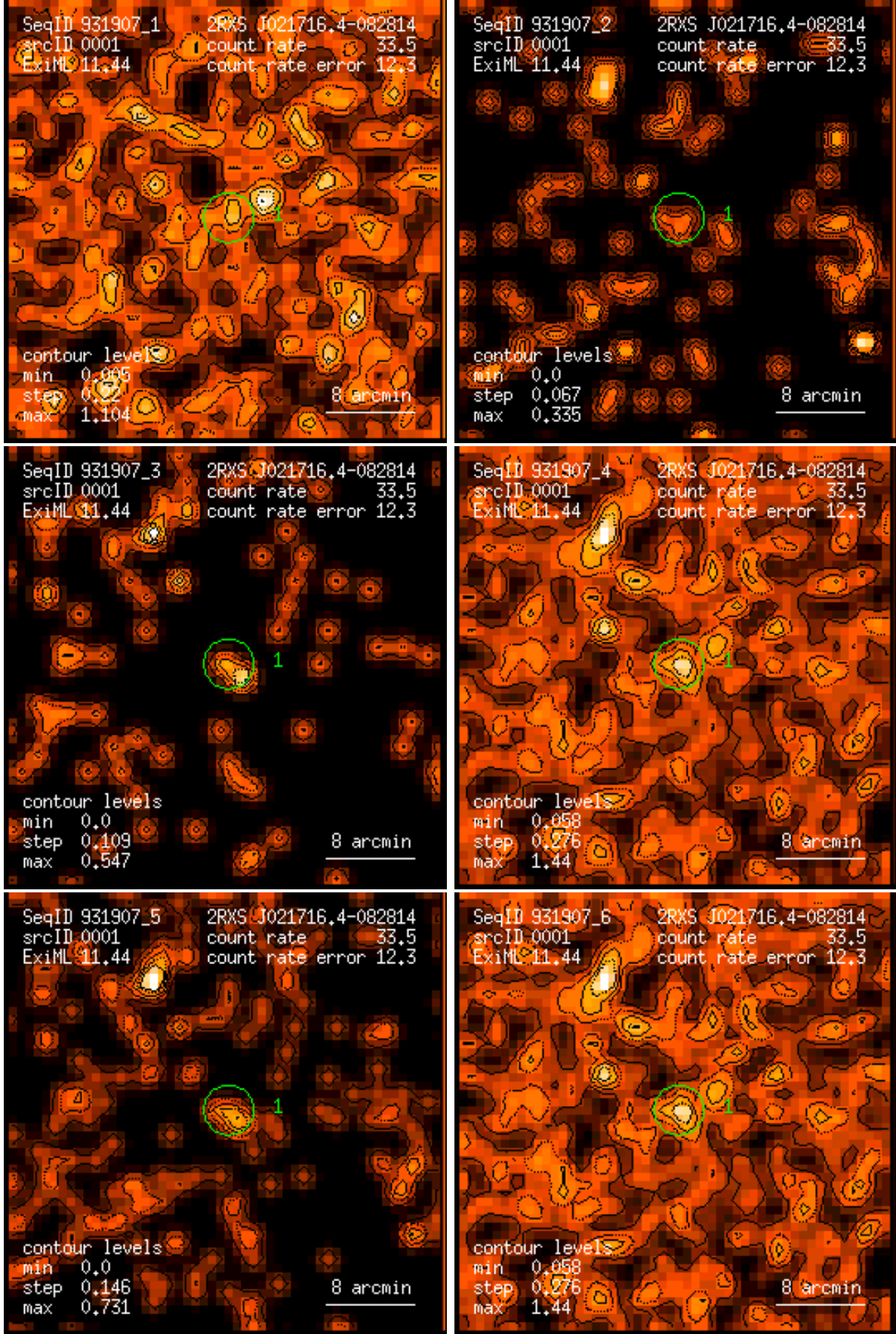
Figure 1: RASS 931907: detection 0001: band rate images, Gaussian filter: (1) PSPC channels 11 – 41, (2) 52 – 90, (3) 91 – 201, (4) 11 – 235, (5) 52 – 201, (6) 11 – 201. Broad band rates in counts/ks. Band rate contour levels in counts/ks/arcmin 2 .
