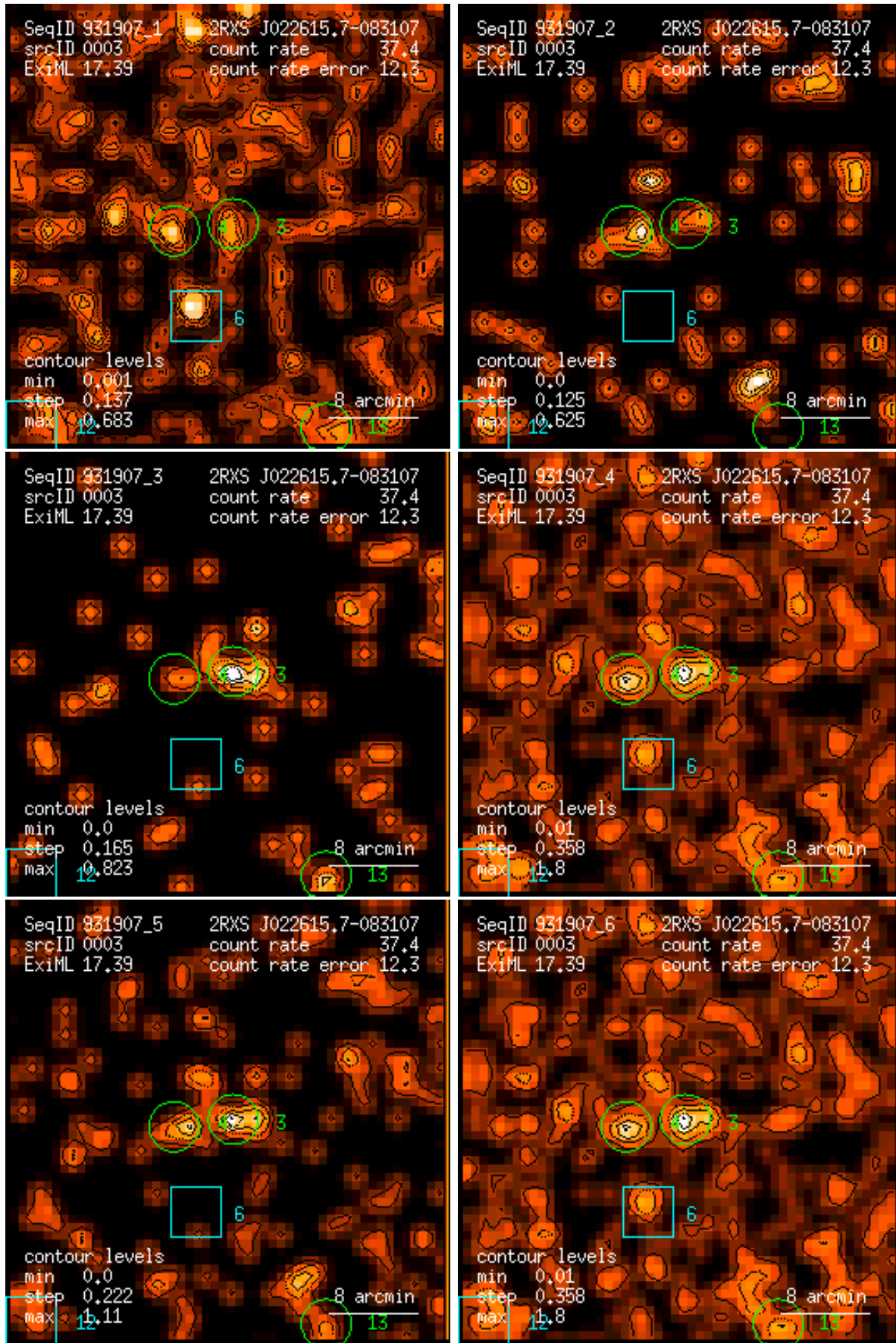
Figure 3: RASS 931907: detection 0003: band rate images, Gaussian filter: (1) PSPC channels 11 – 41, (2) 52 – 90, (3) 91 – 201, (4) 11 – 235, (5) 52 – 201, (6) 11 – 201. Broad band rates in counts/ks. Band rate contour levels in counts/ks/arcmin 2 .
