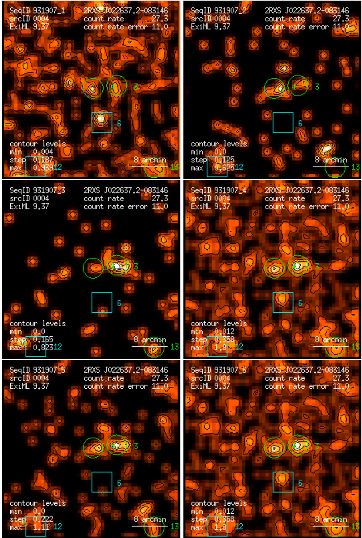
Figure 4: RASS 931907: detection 0004: band rate images, Gaussian filter: (1) PSPC channels 11 – 41, (2) 52 – 90, (3) 91 – 201, (4) 11 – 235, (5) 52 – 201, (6) 11 – 201. Broad band rates in counts/ks. Band rate contour levels in counts/ks/arcmin 2 .
