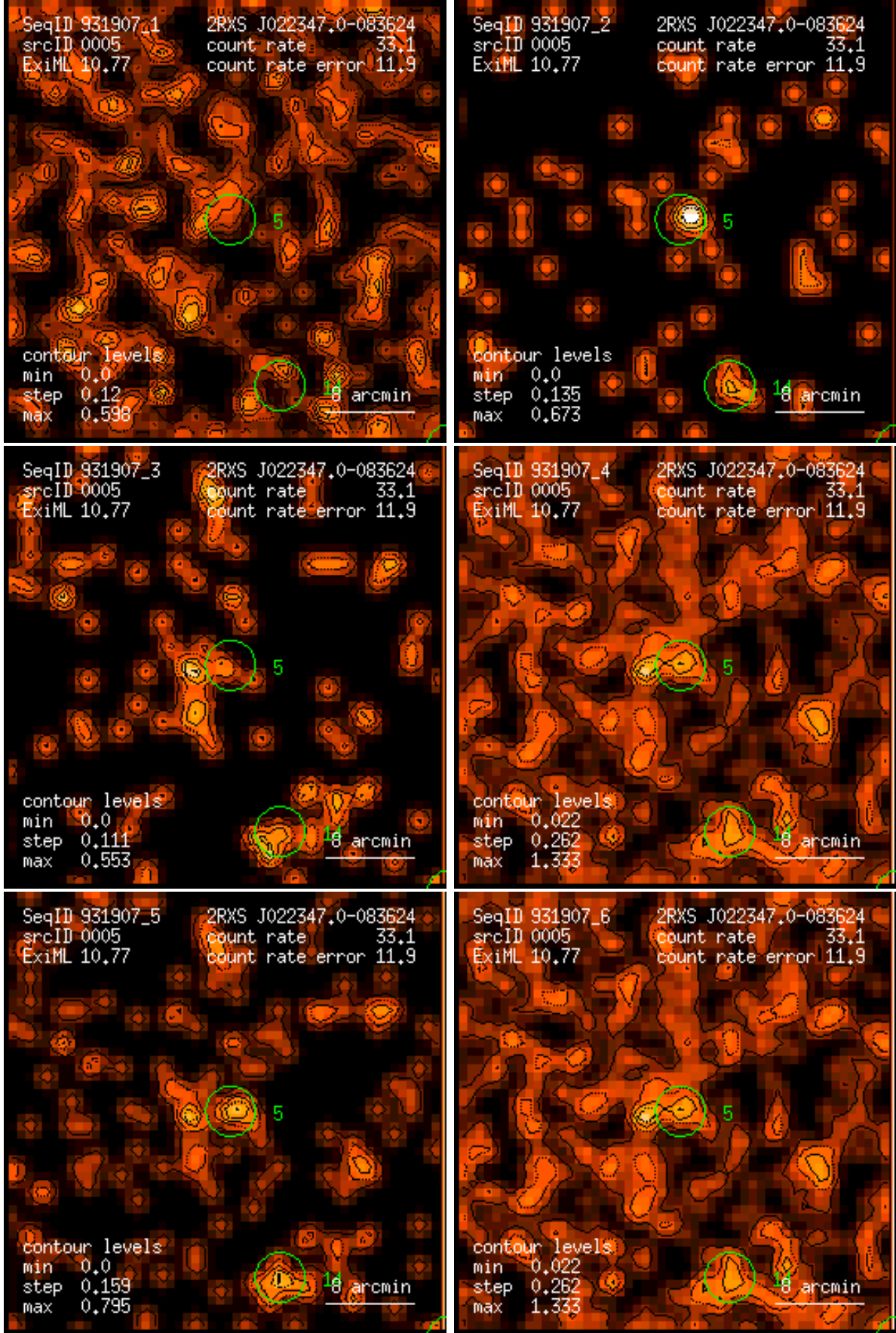
Figure 5: RASS 931907: detection 0005: band rate images, Gaussian filter: (1) PSPC channels 11 – 41, (2) 52 – 90, (3) 91 – 201, (4) 11 – 235, (5) 52 – 201, (6) 11 – 201. Broad band rates in counts/ks. Band rate contour levels in counts/ks/arcmin 2 .
