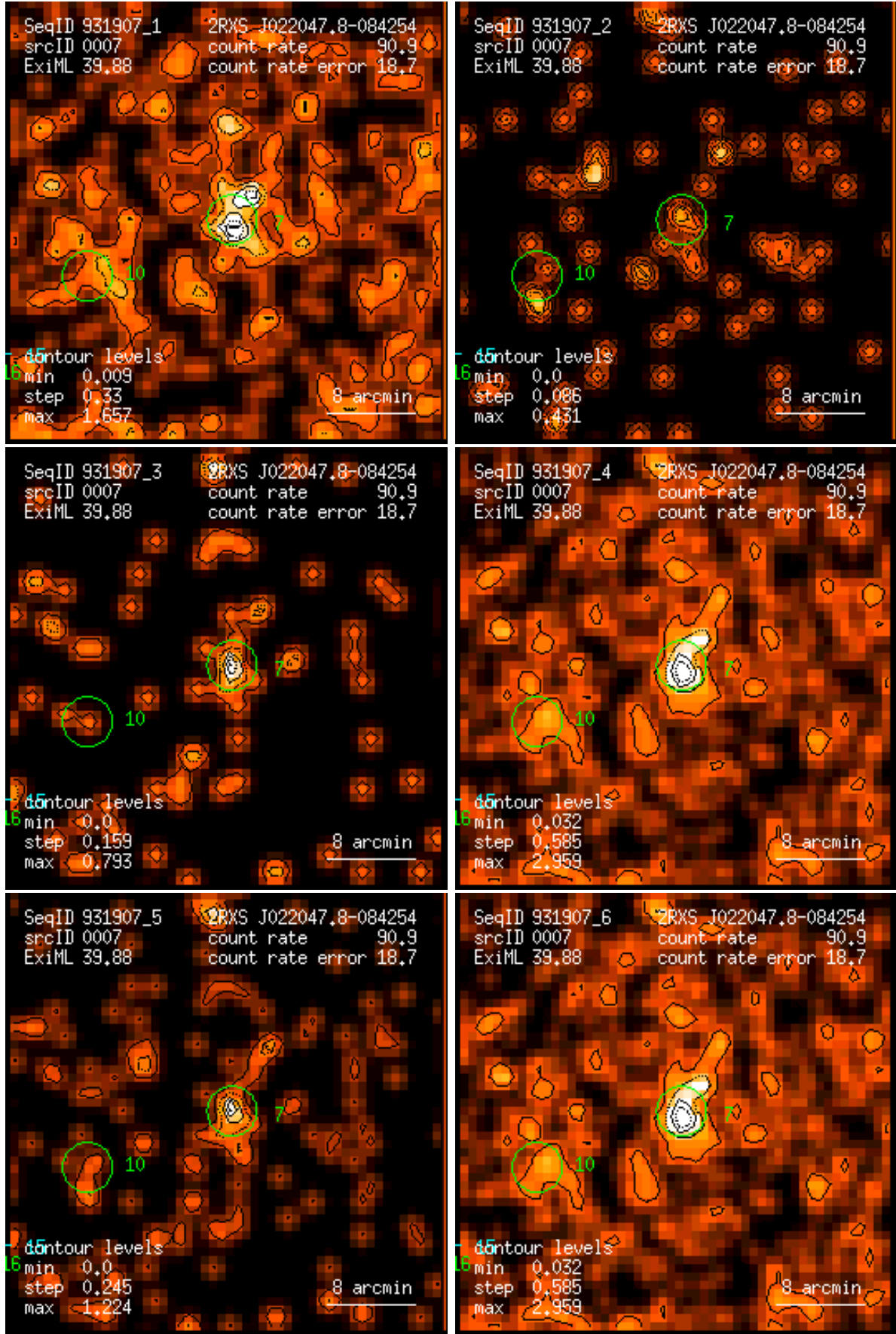
Figure 7: RASS 931907: detection 0007: band rate images, Gaussian filter: (1) PSPC channels 11 – 41, (2) 52 – 90, (3) 91 – 201, (4) 11 – 235, (5) 52 – 201, (6) 11 – 201. Broad band rates in counts/ks. Band rate contour levels in counts/ks/arcmin 2 .
